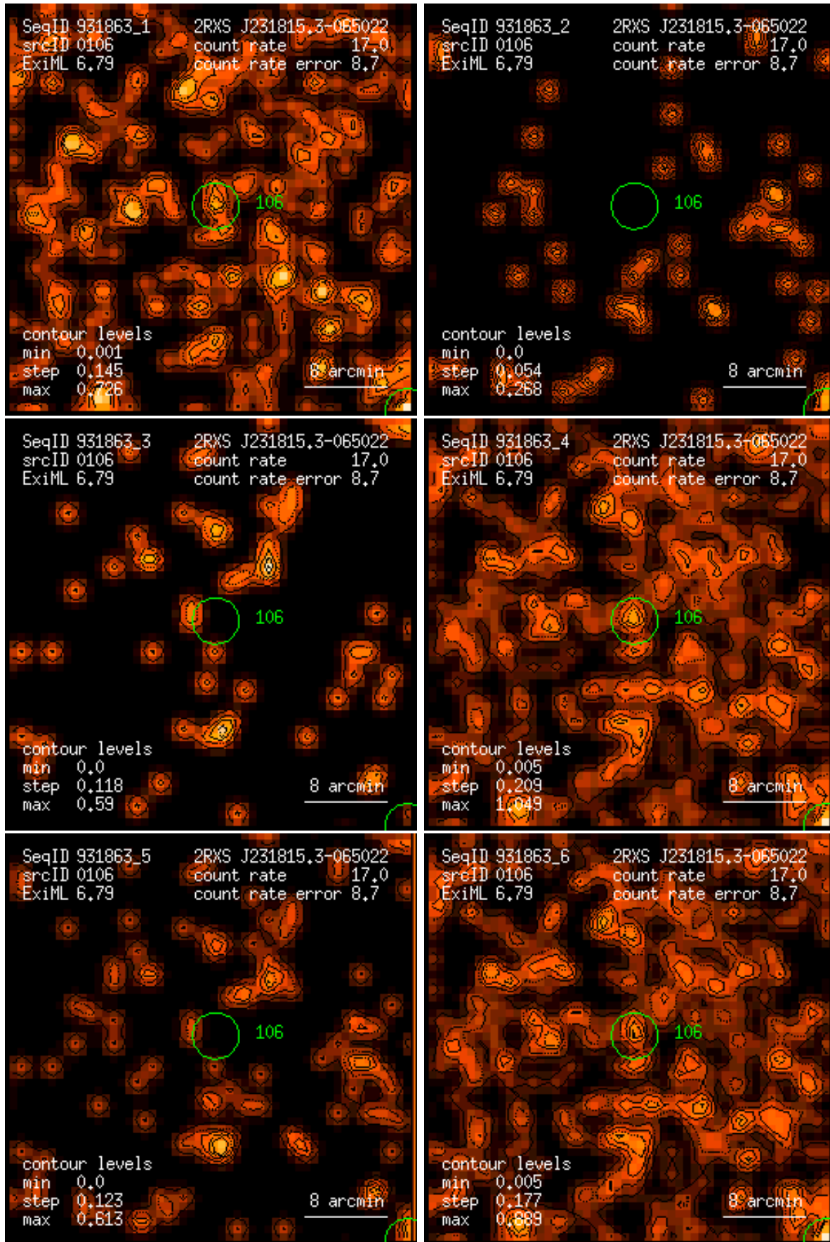
Figure 106: RASS 931863: detection 0106: band rate images, Gaussian filter: (1) PSPC channels 11 – 41, (2) 52 – 90, (3) 91 – 201, (4) 11 – 235, (5) 52 – 201, (6) 11 – 201. Broad band rates in counts/ks. Band rate contour levels in counts/ks/arcmin 2 .
