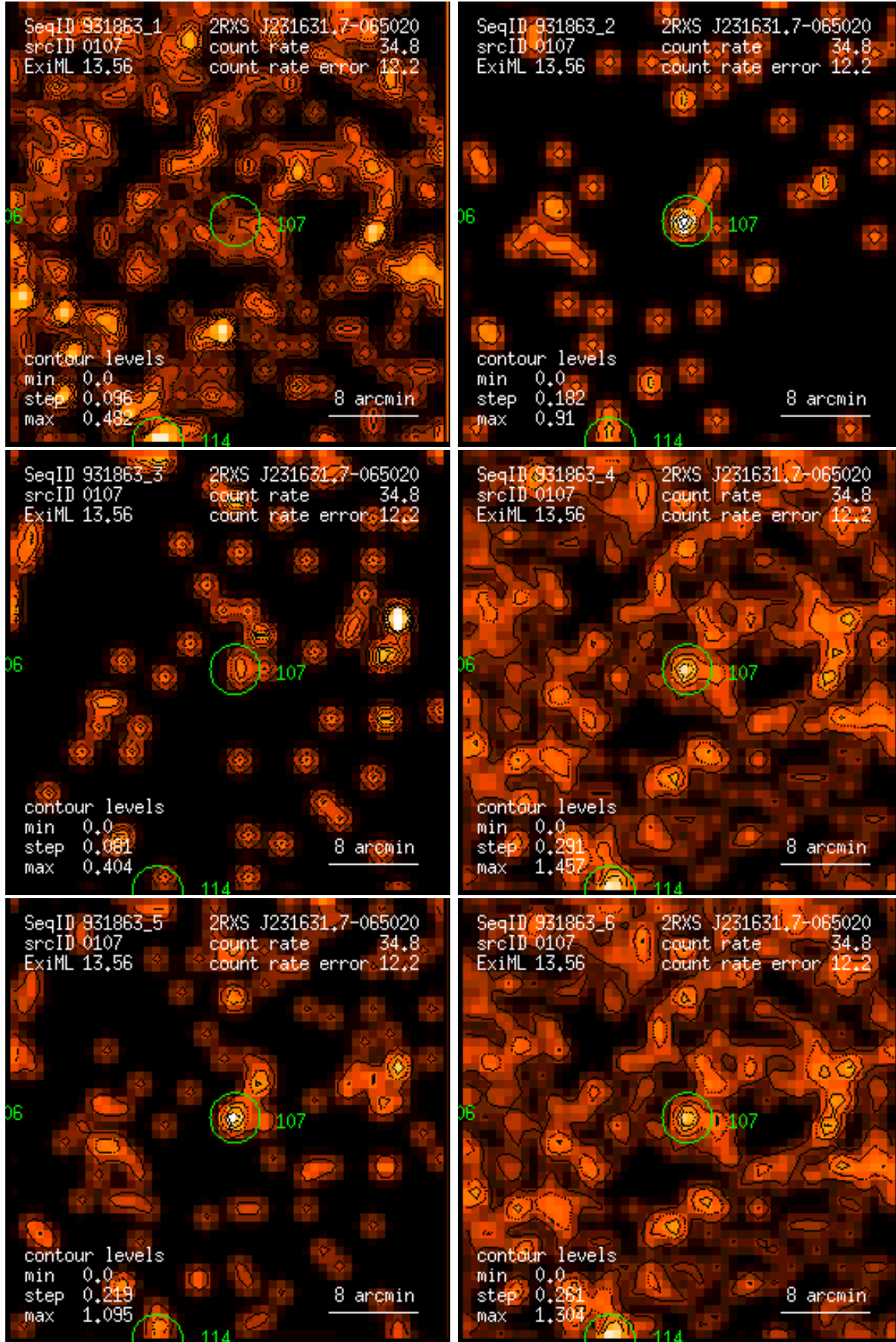
Figure 107: RASS 931863: detection 0107: band rate images, Gaussian filter: (1) PSPC channels 11 – 41, (2) 52 – 90, (3) 91 – 201, (4) 11 – 235, (5) 52 – 201, (6) 11 – 201. Broad band rates in counts/ks. Band rate contour levels in counts/ks/arcmin 2 .
