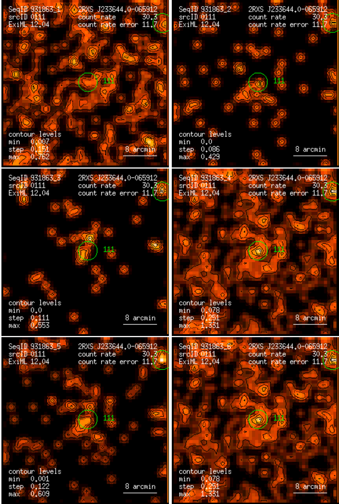
Figure 111: RASS 931863: detection 0111: band rate images, Gaussian filter: (1) PSPC channels 11 – 41, (2) 52 – 90, (3) 91 – 201, (4) 11 – 235, (5) 52 – 201, (6) 11 – 201. Broad band rates in counts/ks. Band rate contour levels in counts/ks/arcmin 2 .
