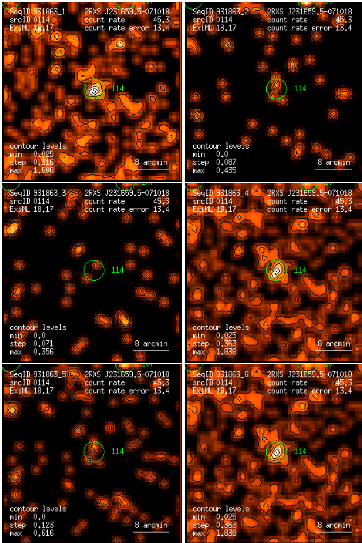
Figure 114: RASS 931863: detection 0114: band rate images, Gaussian filter: (1) PSPC channels 11 – 41, (2) 52 – 90, (3) 91 – 201, (4) 11 – 235, (5) 52 – 201, (6) 11 – 201. Broad band rates in counts/ks. Band rate contour levels in counts/ks/arcmin 2 .
