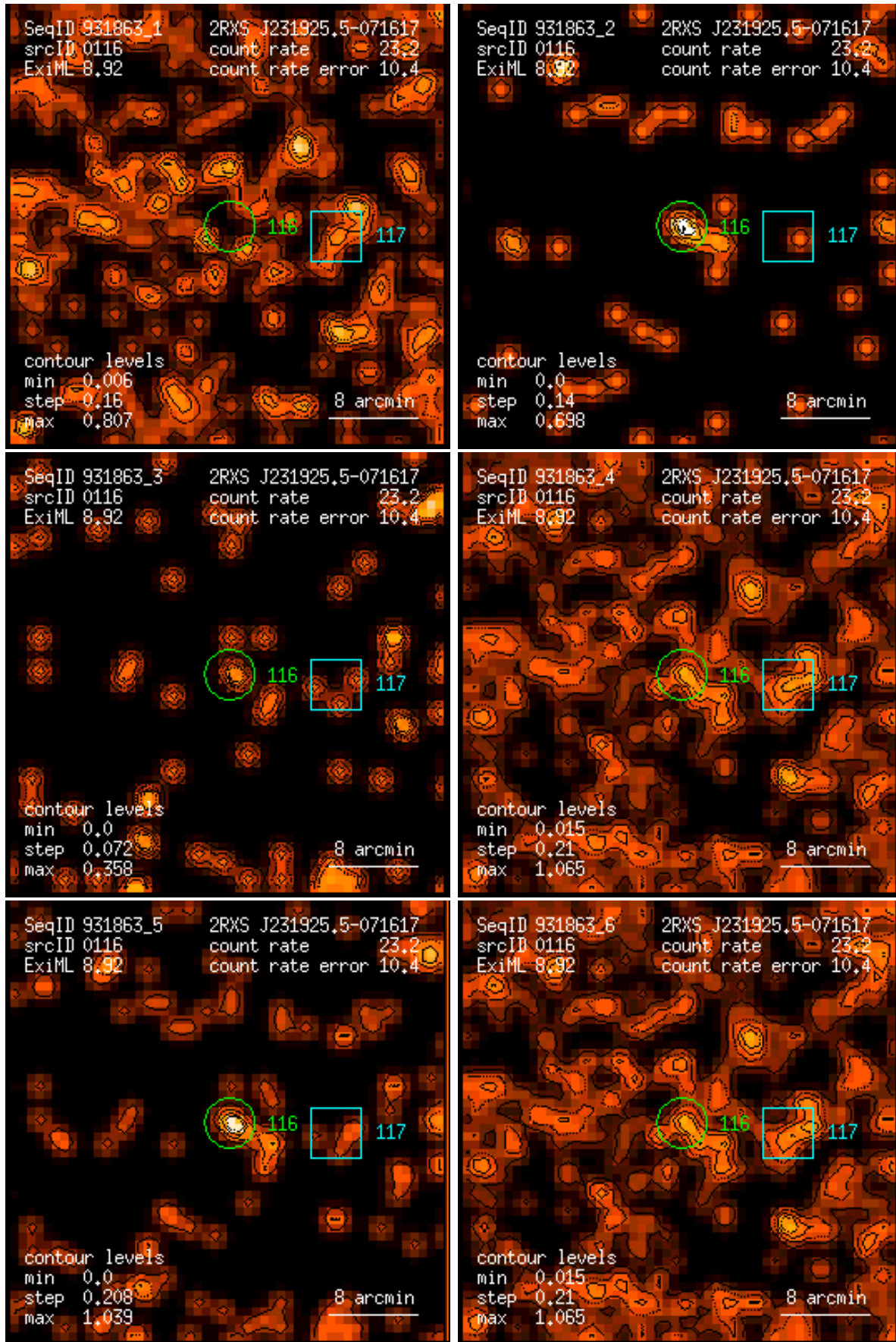
Figure 116: RASS 931863: detection 0116: band rate images, Gaussian filter: (1) PSPC channels 11 – 41, (2) 52 – 90, (3) 91 – 201, (4) 11 – 235, (5) 52 – 201, (6) 11 – 201. Broad band rates in counts/ks. Band rate contour levels in counts/ks/arcmin 2 .
