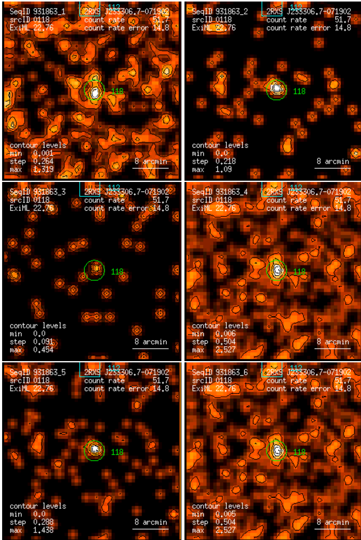
Figure 118: RASS 931863: detection 0118: band rate images, Gaussian filter: (1) PSPC channels 11 – 41, (2) 52 – 90, (3) 91 – 201, (4) 11 – 235, (5) 52 – 201, (6) 11 – 201. Broad band rates in counts/ks. Band rate contour levels in counts/ks/arcmin 2 .
