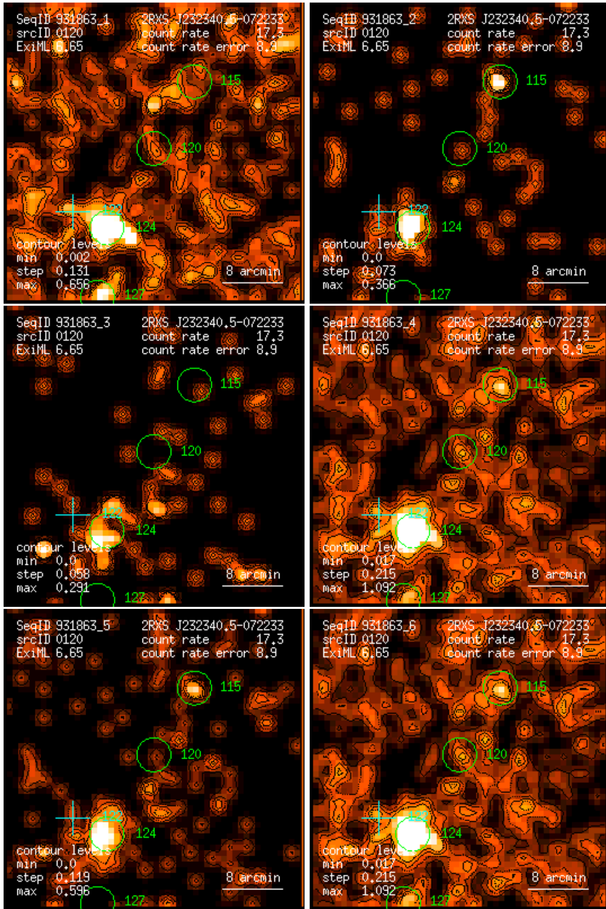
Figure 120: RASS 931863: detection 0120: band rate images, Gaussian filter: (1) PSPC channels 11 – 41, (2) 52 – 90, (3) 91 – 201, (4) 11 – 235, (5) 52 – 201, (6) 11 – 201. Broad band rates in counts/ks. Band rate contour levels in counts/ks/arcmin 2 .
