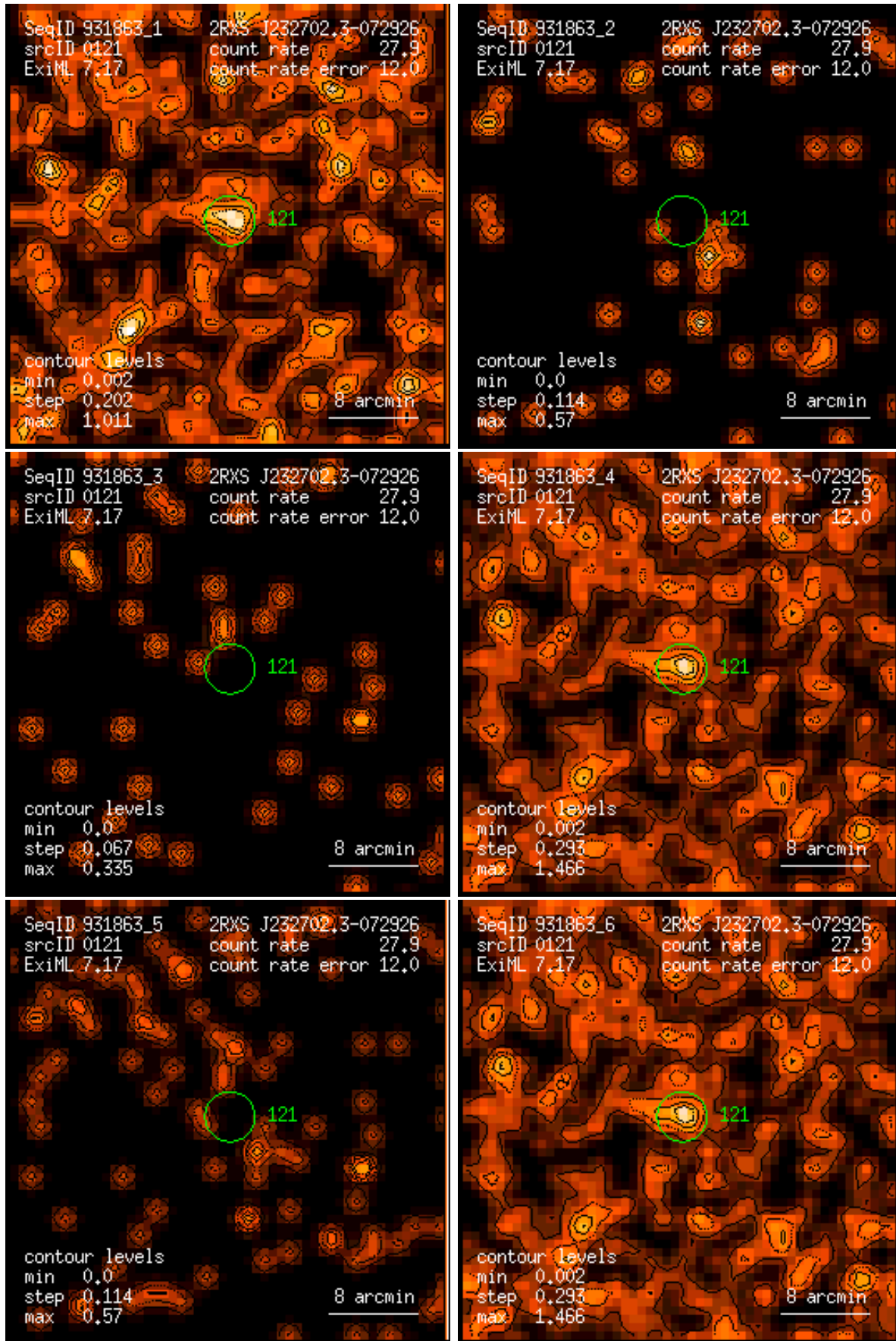
Figure 121: RASS 931863: detection 0121: band rate images, Gaussian filter: (1) PSPC channels 11 – 41, (2) 52 – 90, (3) 91 – 201, (4) 11 – 235, (5) 52 – 201, (6) 11 – 201. Broad band rates in counts/ks. Band rate contour levels in counts/ks/arcmin 2 .
