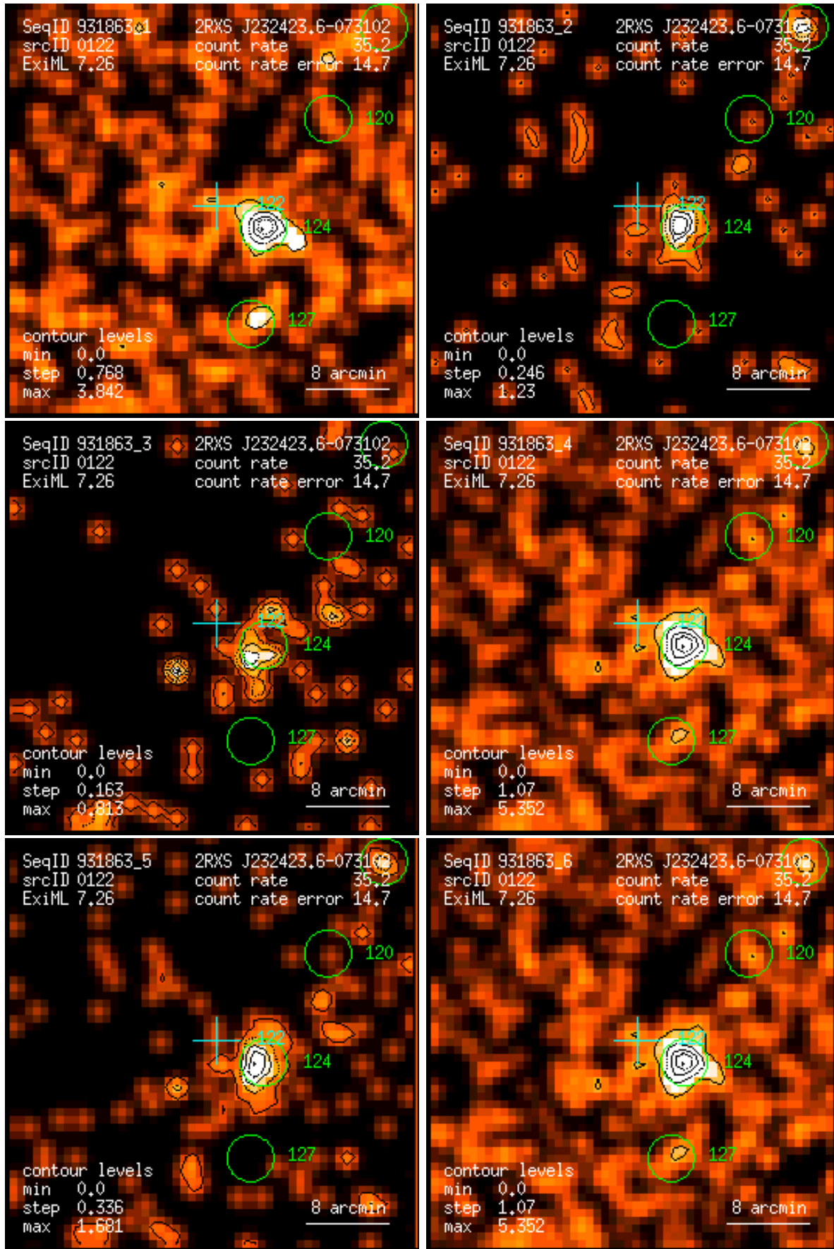
Figure 122: RASS 931863: detection 0122: band rate images, Gaussian filter: (1) PSPC channels 11 – 41, (2) 52 – 90, (3) 91 – 201, (4) 11 – 235, (5) 52 – 201, (6) 11 – 201. Broad band rates in counts/ks. Band rate contour levels in counts/ks/arcmin 2 .
