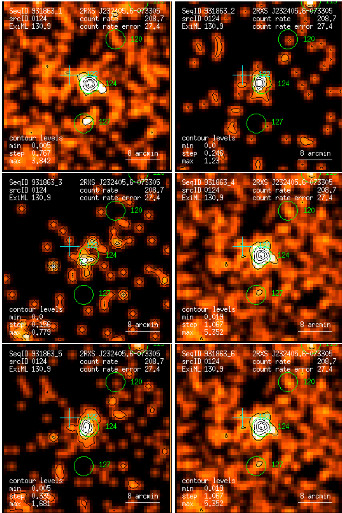
Figure 124: RASS 931863: detection 0124: band rate images, Gaussian filter: (1) PSPC channels 11 – 41, (2) 52 – 90, (3) 91 – 201, (4) 11 – 235, (5) 52 – 201, (6) 11 – 201. Broad band rates in counts/ks. Band rate contour levels in counts/ks/arcmin 2 .
