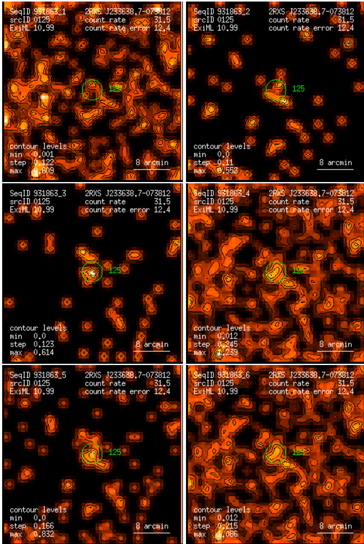
Figure 125: RASS 931863: detection 0125: band rate images, Gaussian filter: (1) PSPC channels 11 – 41, (2) 52 – 90, (3) 91 – 201, (4) 11 – 235, (5) 52 – 201, (6) 11 – 201. Broad band rates in counts/ks. Band rate contour levels in counts/ks/arcmin 2 .
