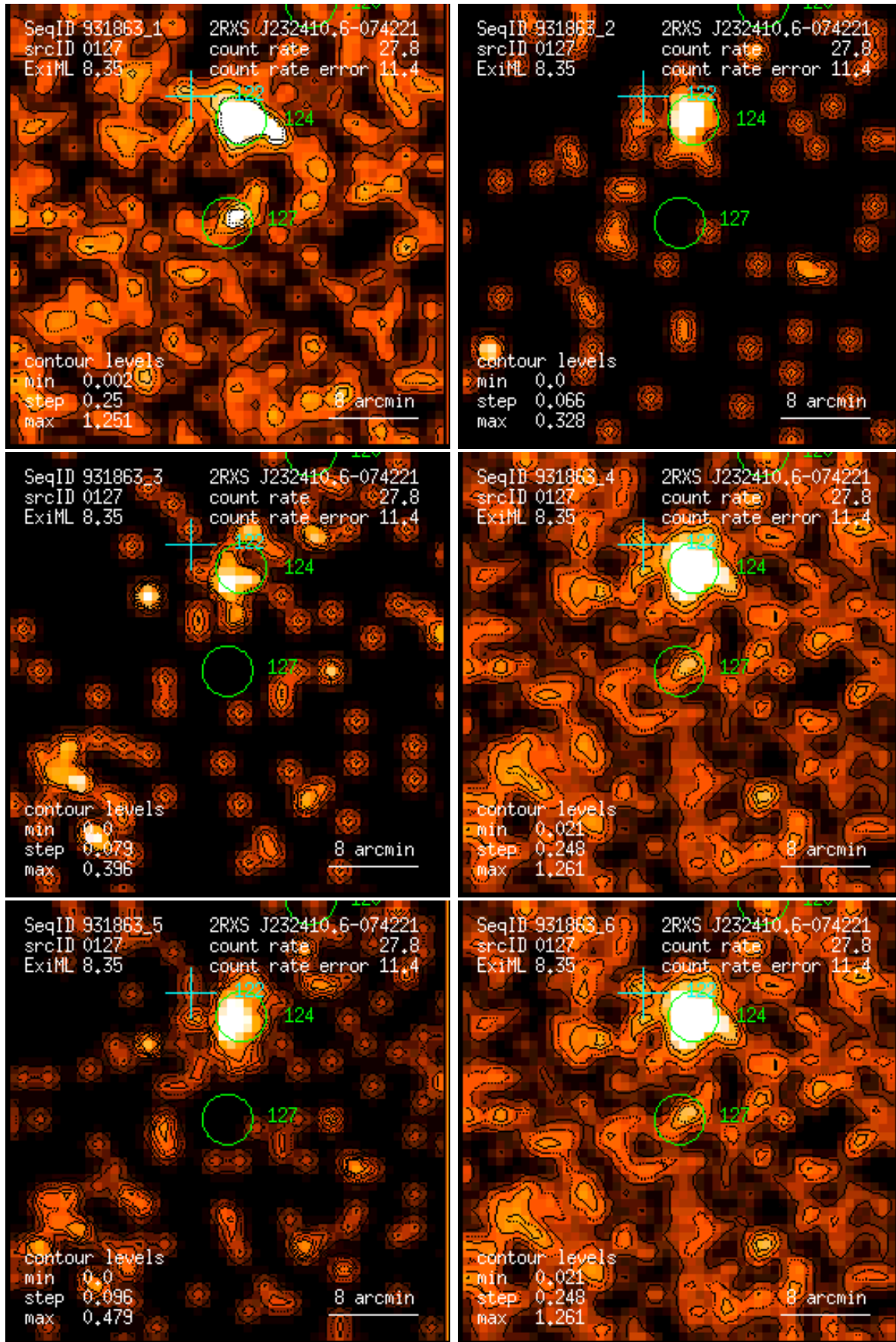
Figure 127: RASS 931863: detection 0127: band rate images, Gaussian filter: (1) PSPC channels 11 – 41, (2) 52 – 90, (3) 91 – 201, (4) 11 – 235, (5) 52 – 201, (6) 11 – 201. Broad band rates in counts/ks. Band rate contour levels in counts/ks/arcmin 2 .
