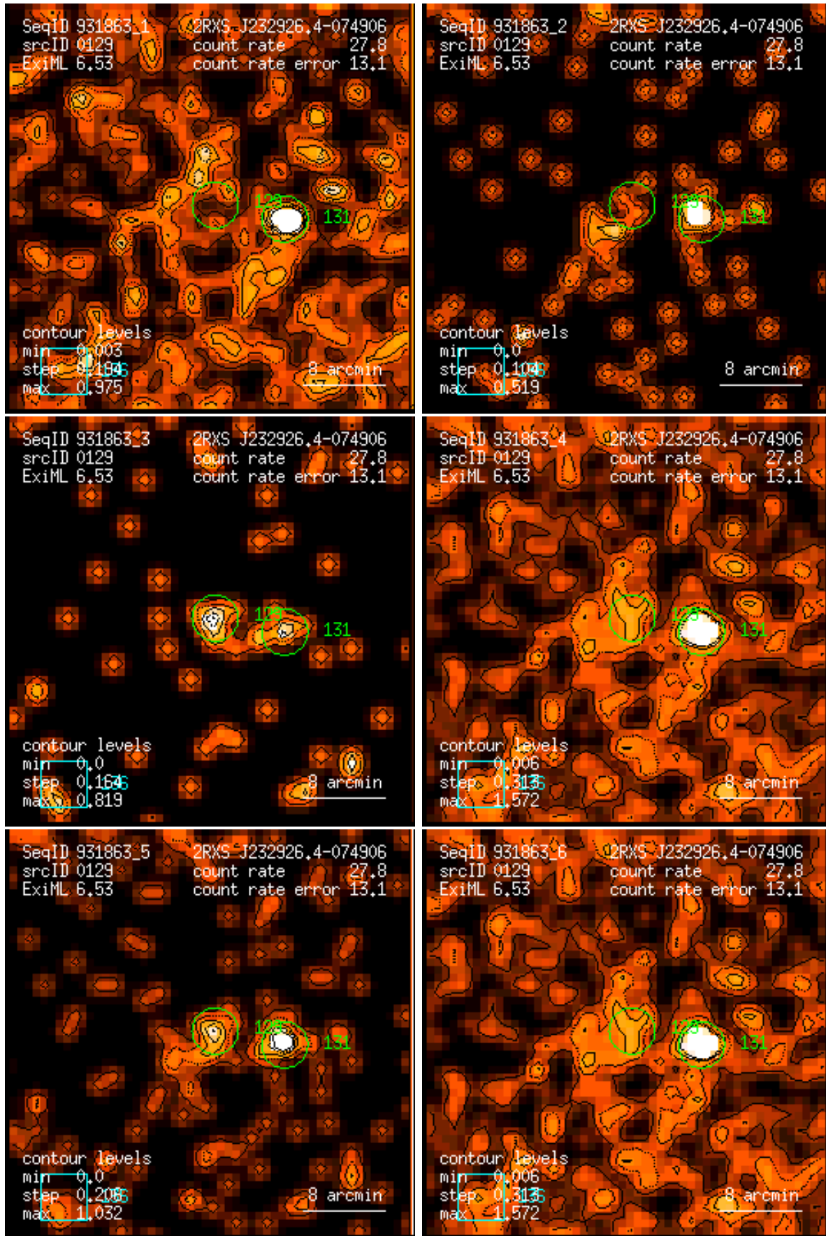
Figure 129: RASS 931863: detection 0129: band rate images, Gaussian filter: (1) PSPC channels 11 – 41, (2) 52 – 90, (3) 91 – 201, (4) 11 – 235, (5) 52 – 201, (6) 11 – 201. Broad band rates in counts/ks. Band rate contour levels in counts/ks/arcmin 2 .
