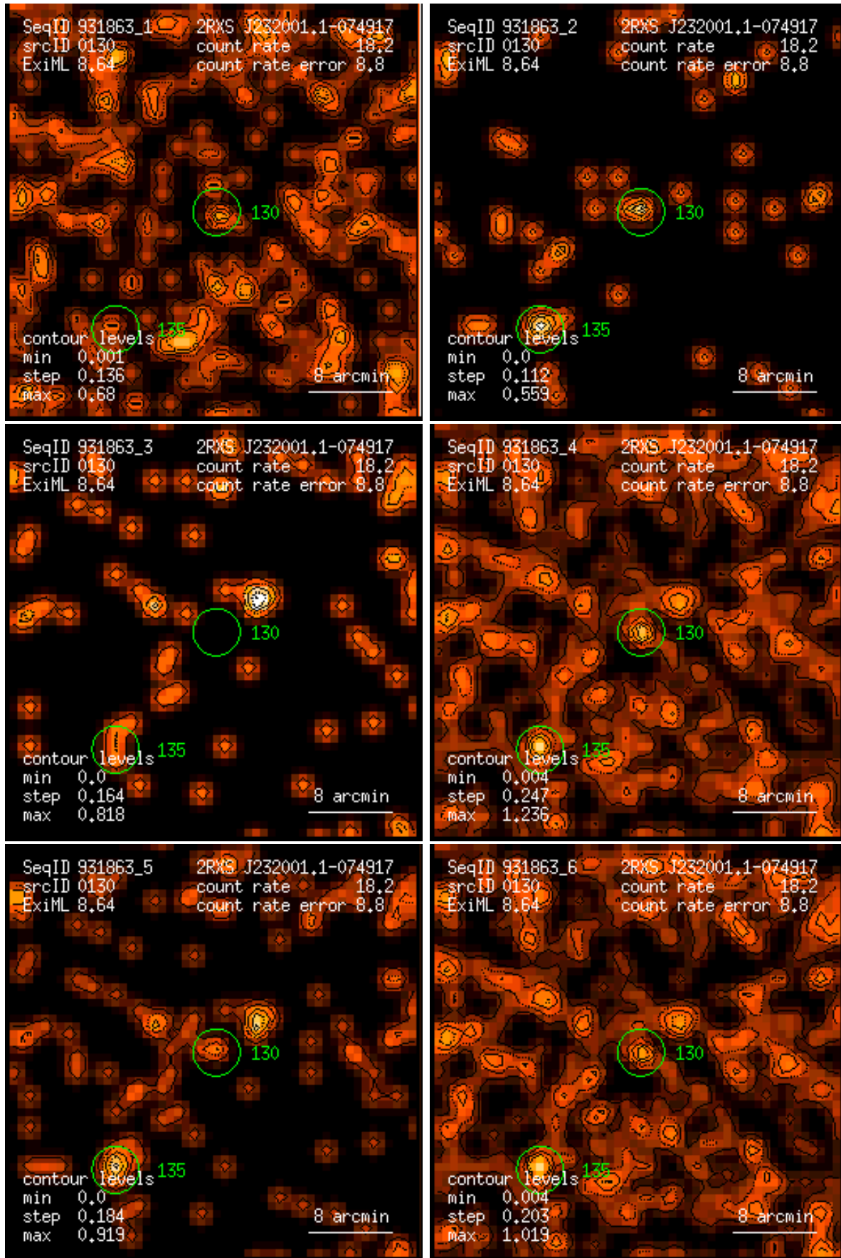
Figure 130: RASS 931863: detection 0130: band rate images, Gaussian filter: (1) PSPC channels 11 – 41, (2) 52 – 90, (3) 91 – 201, (4) 11 – 235, (5) 52 – 201, (6) 11 – 201. Broad band rates in counts/ks. Band rate contour levels in counts/ks/arcmin 2 .
