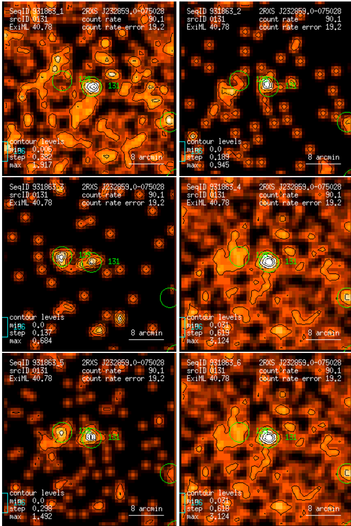
Figure 131: RASS 931863: detection 0131: band rate images, Gaussian filter: (1) PSPC channels 11 – 41, (2) 52 – 90, (3) 91 – 201, (4) 11 – 235, (5) 52 – 201, (6) 11 – 201. Broad band rates in counts/ks. Band rate contour levels in counts/ks/arcmin 2 .
