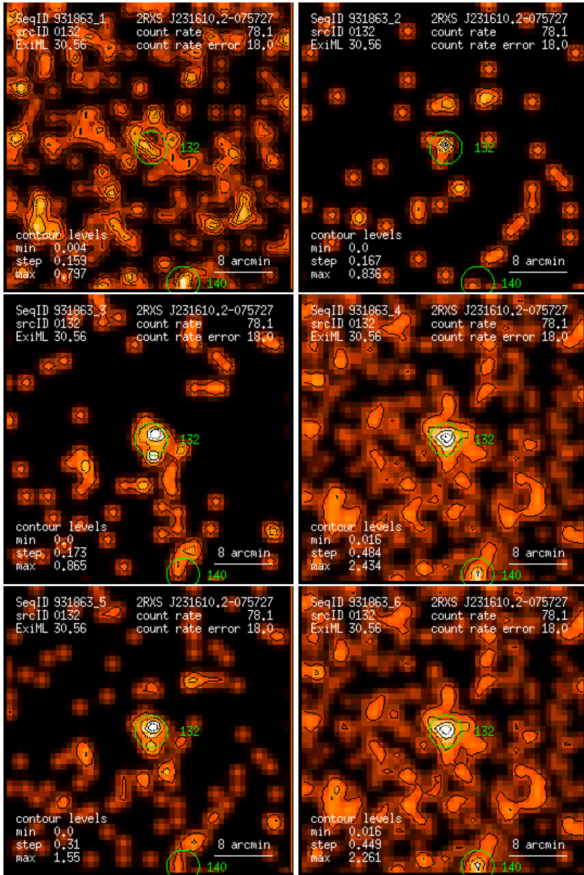
Figure 132: RASS 931863: detection 0132: band rate images, Gaussian filter: (1) PSPC channels 11 – 41, (2) 52 – 90, (3) 91 – 201, (4) 11 – 235, (5) 52 – 201, (6) 11 – 201. Broad band rates in counts/ks. Band rate contour levels in counts/ks/arcmin 2 .
