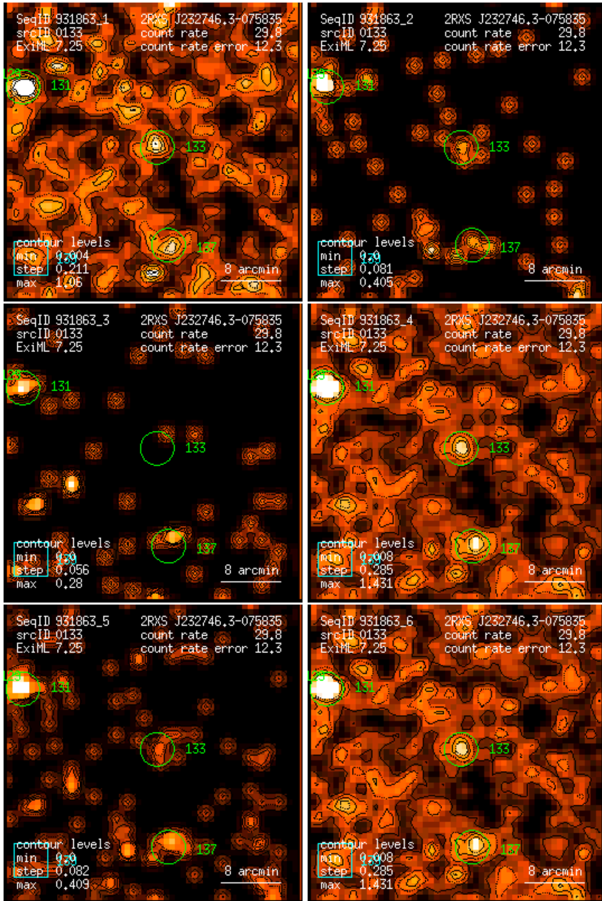
Figure 133: RASS 931863: detection 0133: band rate images, Gaussian filter: (1) PSPC channels 11 – 41, (2) 52 – 90, (3) 91 – 201, (4) 11 – 235, (5) 52 – 201, (6) 11 – 201. Broad band rates in counts/ks. Band rate contour levels in counts/ks/arcmin 2 .
