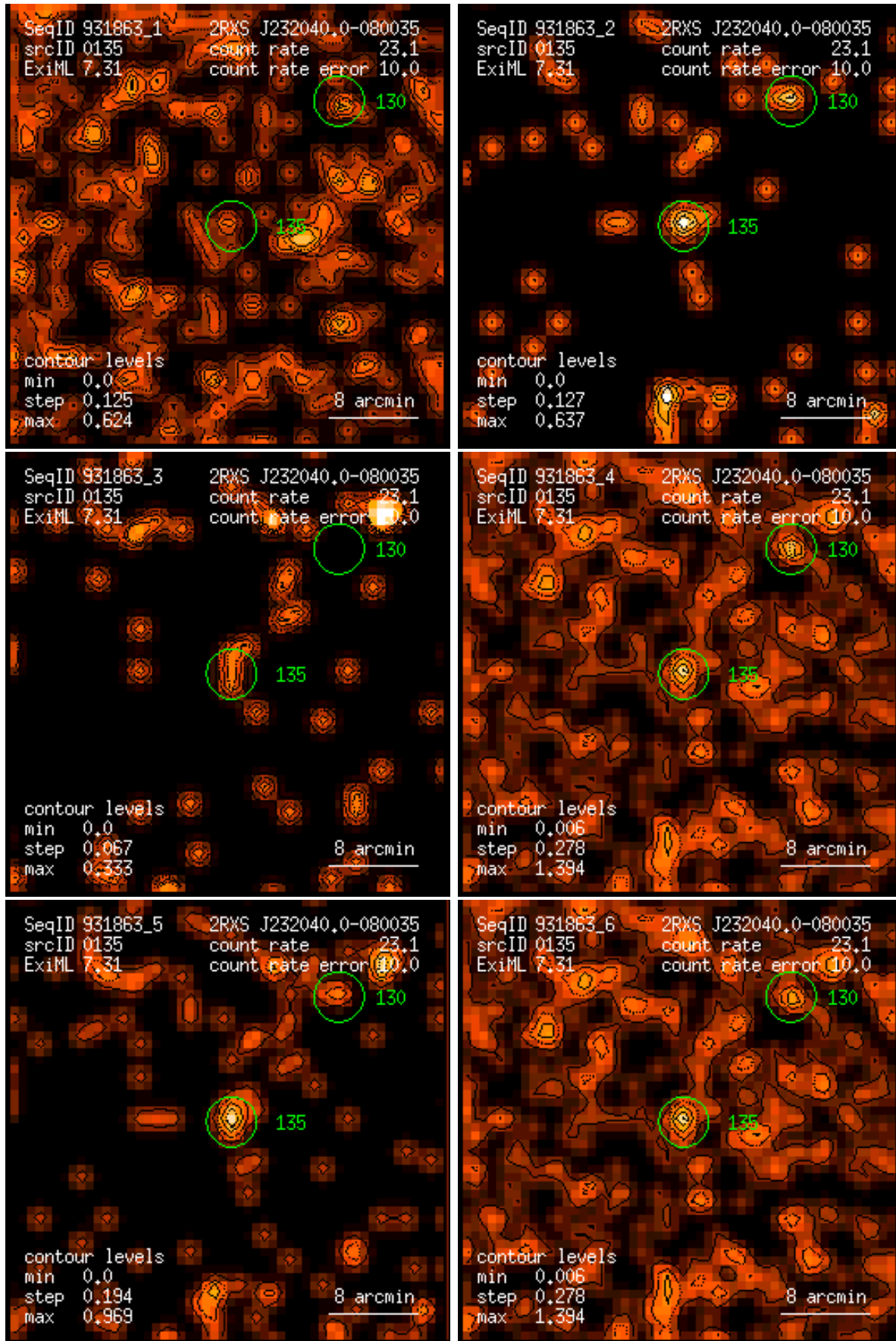
Figure 135: RASS 931863: detection 0135: band rate images, Gaussian filter: (1) PSPC channels 11 – 41, (2) 52 – 90, (3) 91 – 201, (4) 11 – 235, (5) 52 – 201, (6) 11 – 201. Broad band rates in counts/ks. Band rate contour levels in counts/ks/arcmin 2 .
