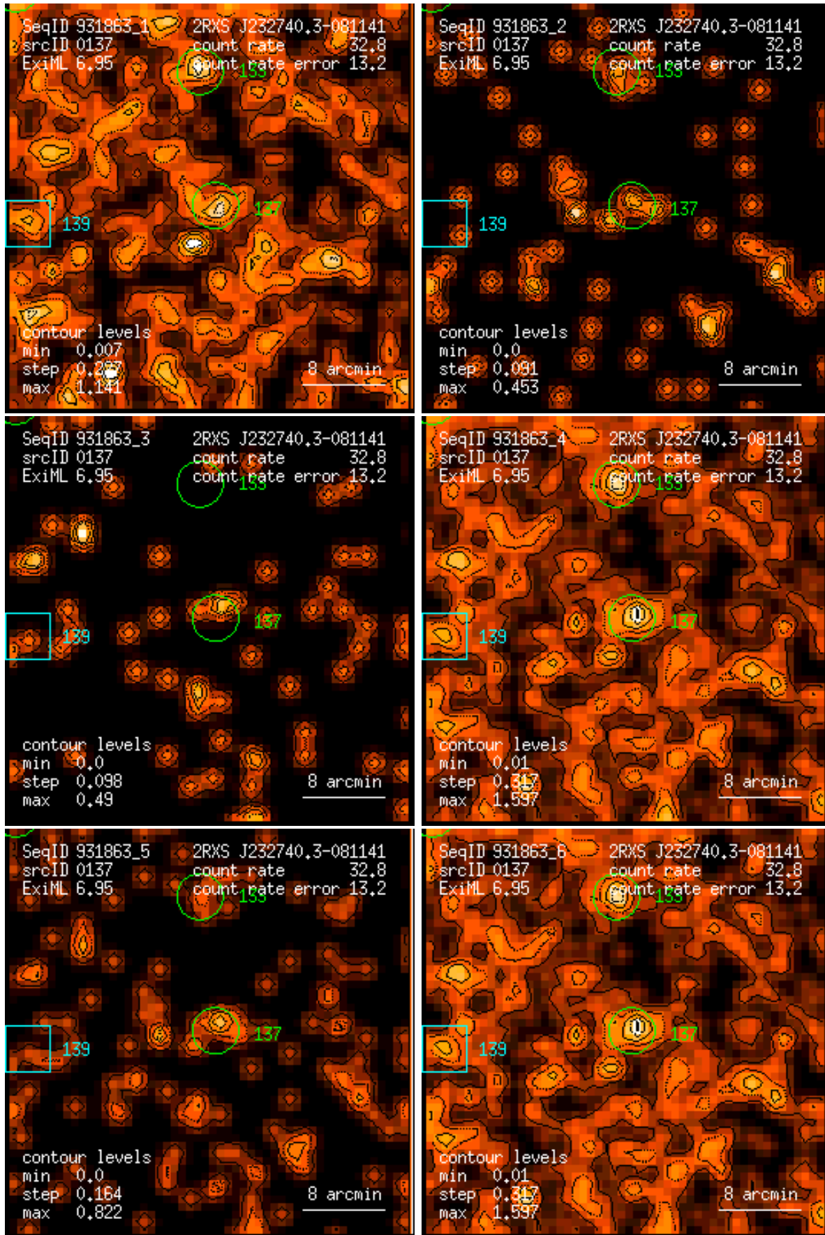
Figure 137: RASS 931863: detection 0137: band rate images, Gaussian filter: (1) PSPC channels 11 – 41, (2) 52 – 90, (3) 91 – 201, (4) 11 – 235, (5) 52 – 201, (6) 11 – 201. Broad band rates in counts/ks. Band rate contour levels in counts/ks/arcmin 2 .
