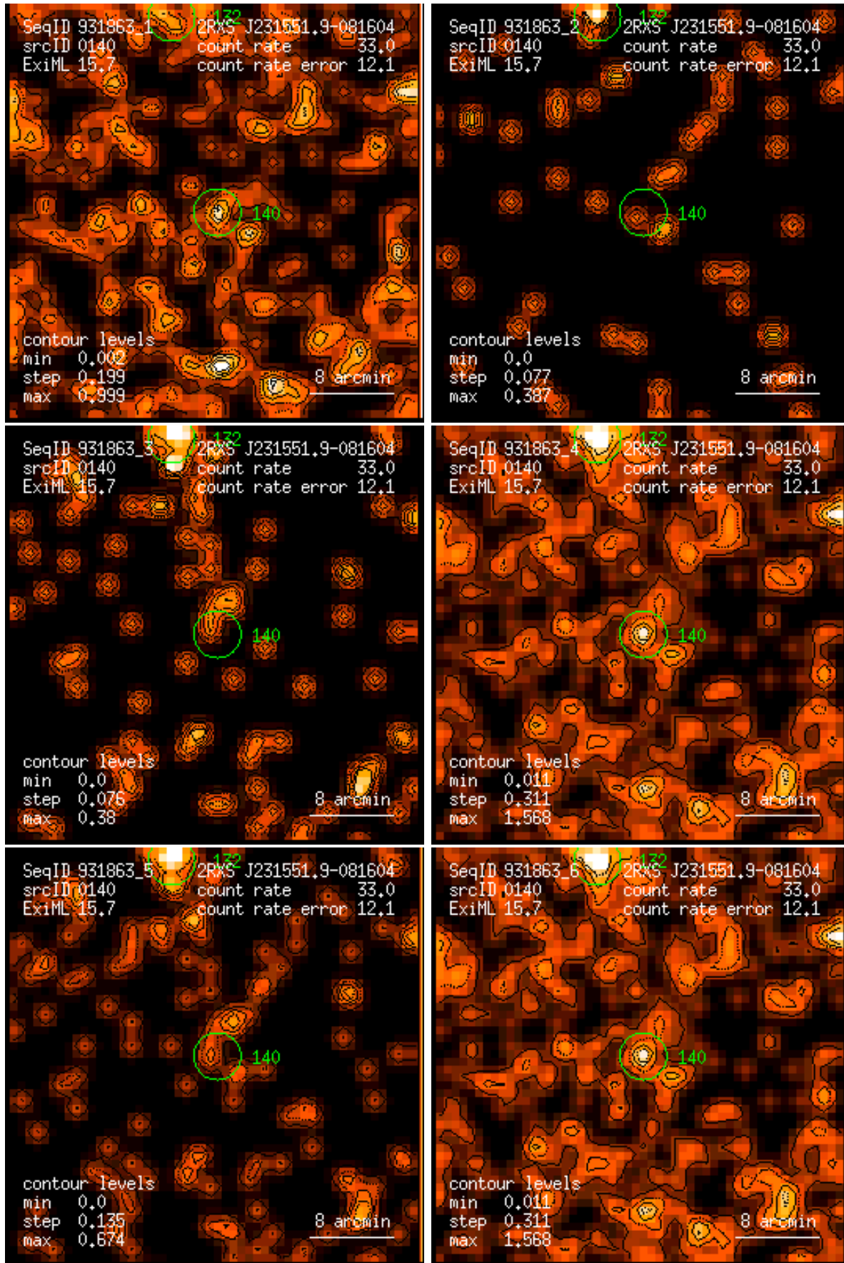
Figure 140: RASS 931863: detection 0140: band rate images, Gaussian filter: (1) PSPC channels 11 – 41, (2) 52 – 90, (3) 91 – 201, (4) 11 – 235, (5) 52 – 201, (6) 11 – 201. Broad band rates in counts/ks. Band rate contour levels in counts/ks/arcmin 2 .
