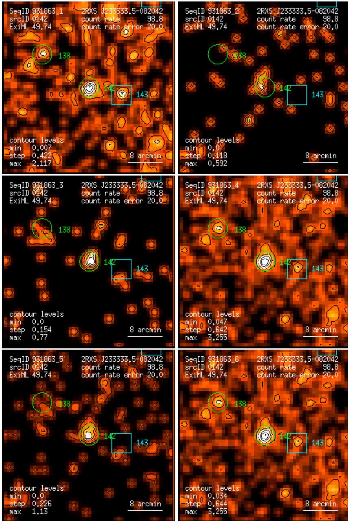
Figure 142: RASS 931863: detection 0142: band rate images, Gaussian filter: (1) PSPC channels 11 – 41, (2) 52 – 90, (3) 91 – 201, (4) 11 – 235, (5) 52 – 201, (6) 11 – 201. Broad band rates in counts/ks. Band rate contour levels in counts/ks/arcmin 2 .
