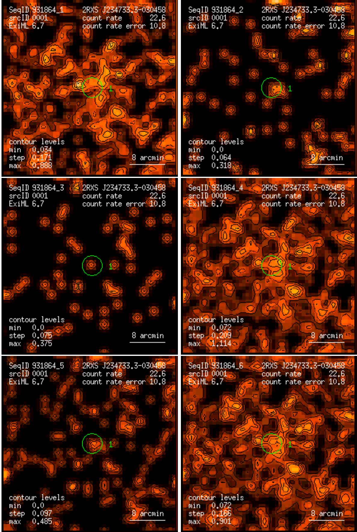
Figure 1: RASS 931864: detection 0001: band rate images, Gaussian filter: (1) PSPC channels 11 – 41, (2) 52 – 90, (3) 91 – 201, (4) 11 – 235, (5) 52 – 201, (6) 11 – 201. Broad band rates in counts/ks. Band rate contour levels in counts/ks/arcmin 2 .
