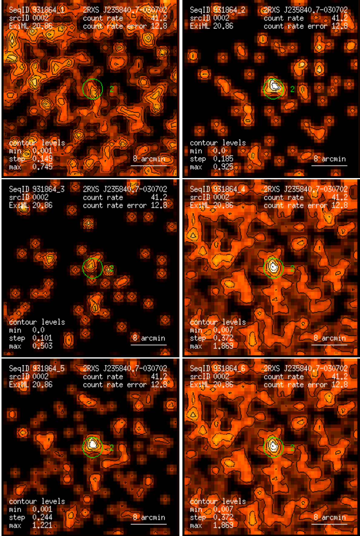
Figure 2: RASS 931864: detection 0002: band rate images, Gaussian filter: (1) PSPC channels 11 – 41, (2) 52 – 90, (3) 91 – 201, (4) 11 – 235, (5) 52 – 201, (6) 11 – 201. Broad band rates in counts/ks. Band rate contour levels in counts/ks/arcmin 2 .
