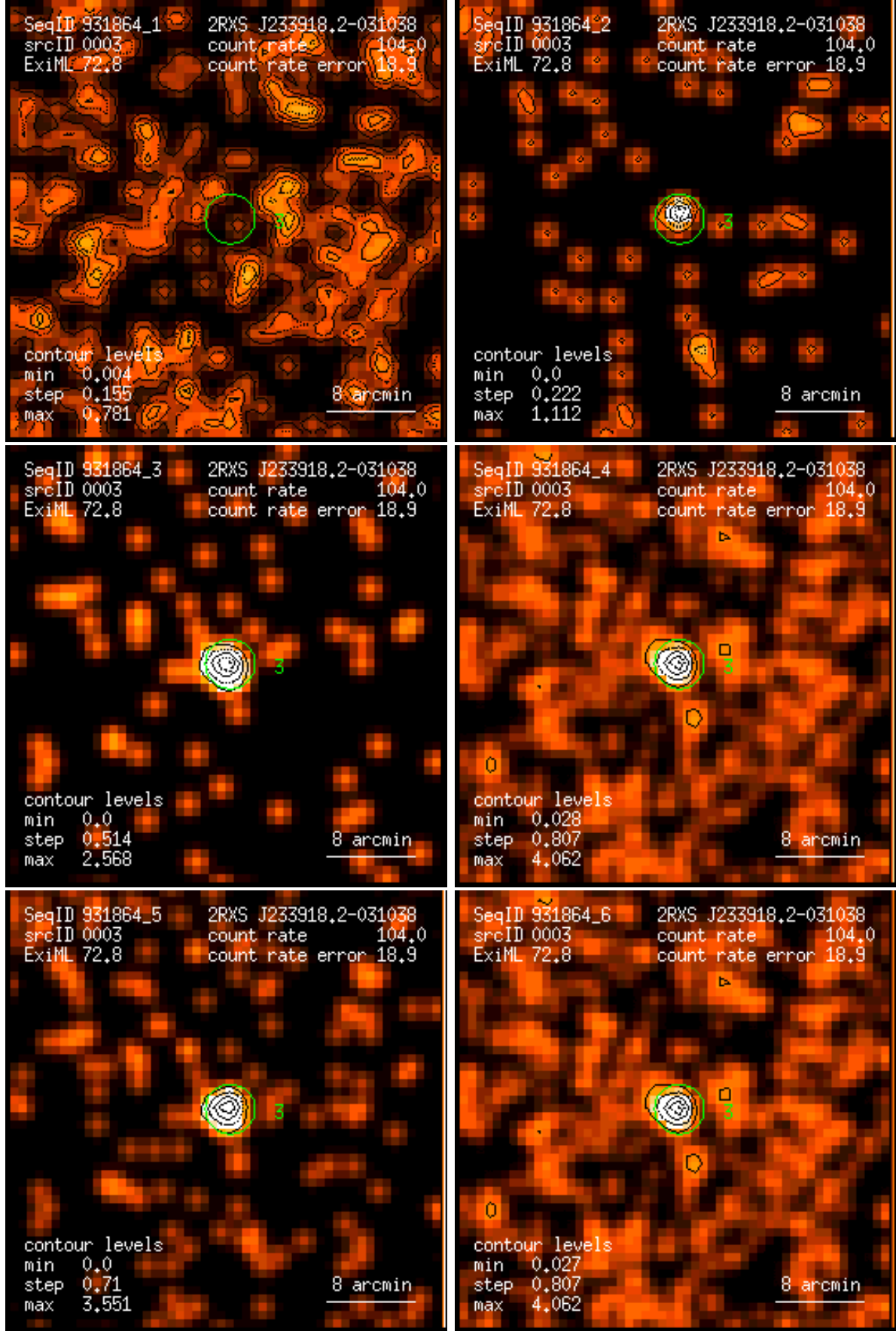
Figure 3: RASS 931864: detection 0003: band rate images, Gaussian filter: (1) PSPC channels 11 – 41, (2) 52 – 90, (3) 91 – 201, (4) 11 – 235, (5) 52 – 201, (6) 11 – 201. Broad band rates in counts/ks. Band rate contour levels in counts/ks/arcmin 2 .
