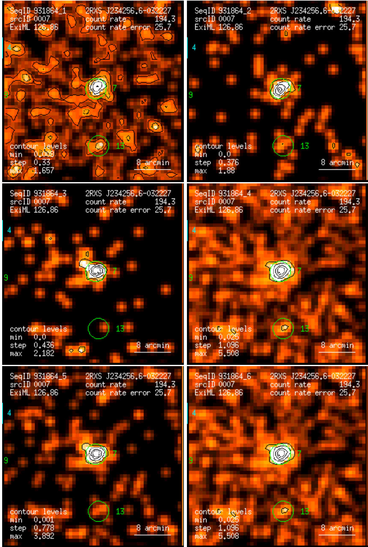
Figure 7: RASS 931864: detection 0007: band rate images, Gaussian filter: (1) PSPC channels 11 – 41, (2) 52 – 90, (3) 91 – 201, (4) 11 – 235, (5) 52 – 201, (6) 11 – 201. Broad band rates in counts/ks. Band rate contour levels in counts/ks/arcmin 2 .
