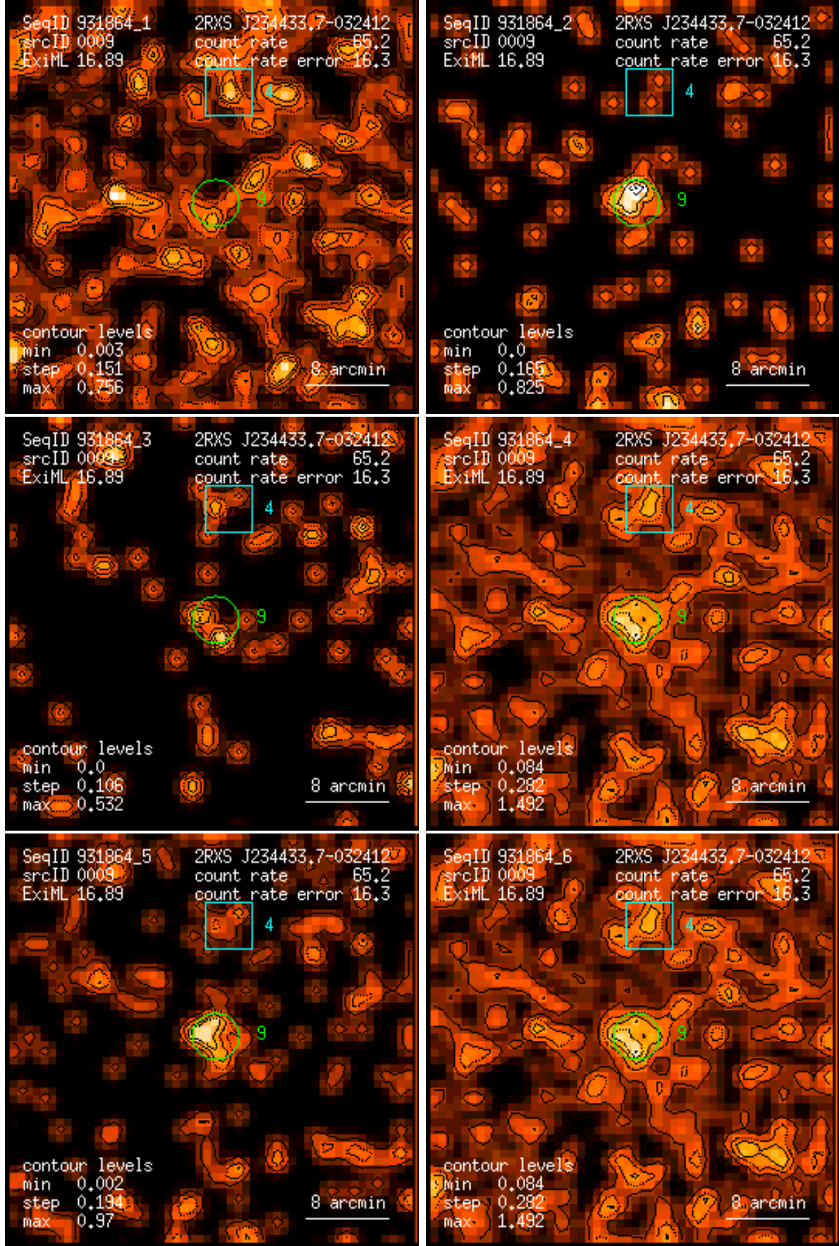
Figure 9: RASS 931864: detection 0009: band rate images, Gaussian filter: (1) PSPC channels 11 – 41, (2) 52 – 90, (3) 91 – 201, (4) 11 – 235, (5) 52 – 201, (6) 11 – 201. Broad band rates in counts/ks. Band rate contour levels in counts/ks/arcmin 2 .
