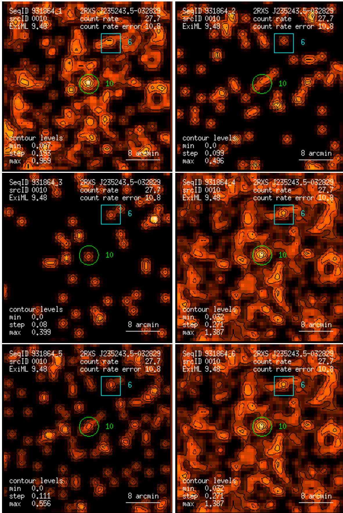
Figure 10: RASS 931864: detection 0010: band rate images, Gaussian filter: (1) PSPC channels 11 – 41, (2) 52 – 90, (3) 91 – 201, (4) 11 – 235, (5) 52 – 201, (6) 11 – 201. Broad band rates in counts/ks. Band rate contour levels in counts/ks/arcmin 2 .
