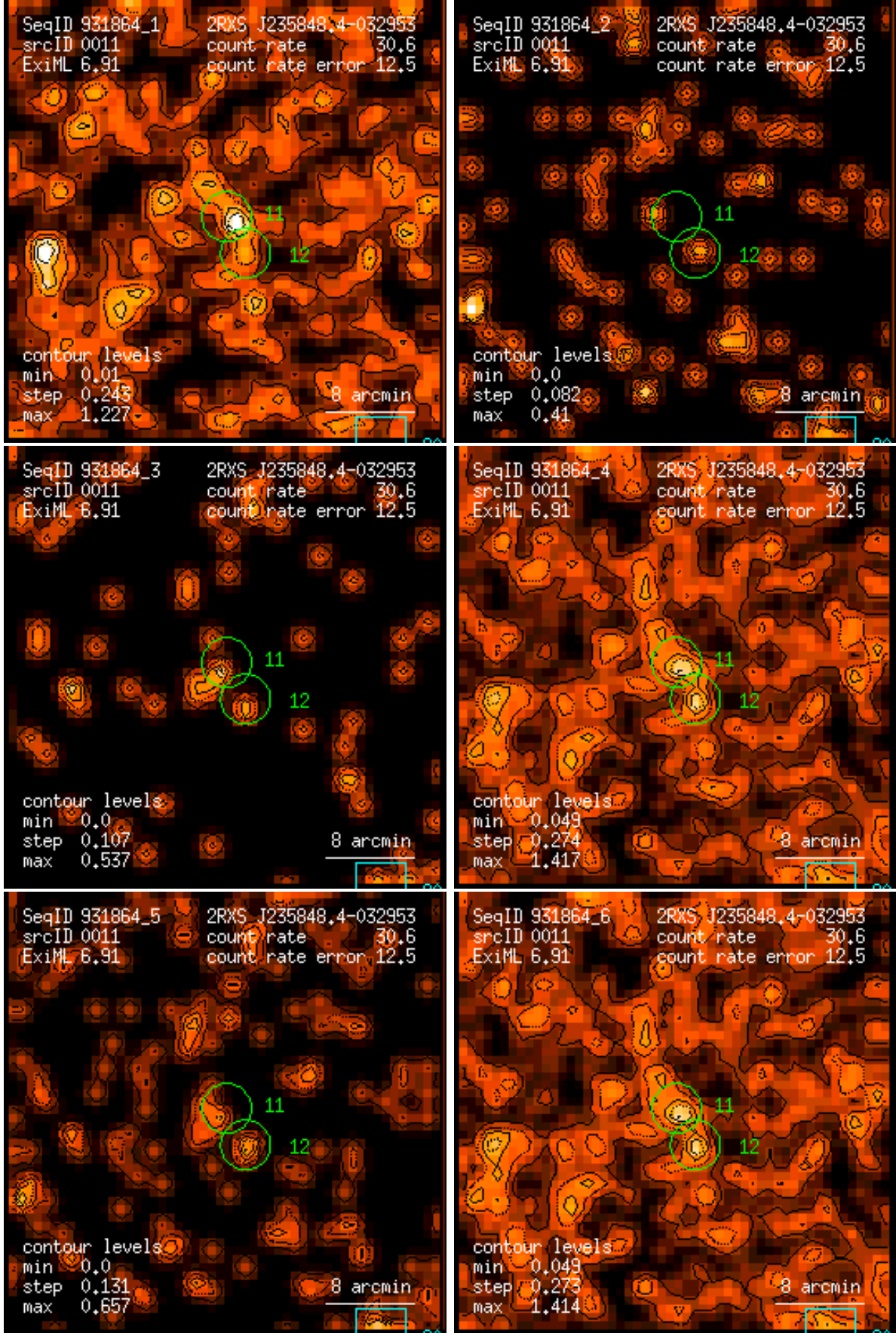
Figure 11: RASS 931864: detection 0011: band rate images, Gaussian filter: (1) PSPC channels 11 – 41, (2) 52 – 90, (3) 91 – 201, (4) 11 – 235, (5) 52 – 201, (6) 11 – 201. Broad band rates in counts/ks. Band rate contour levels in counts/ks/arcmin 2 .
