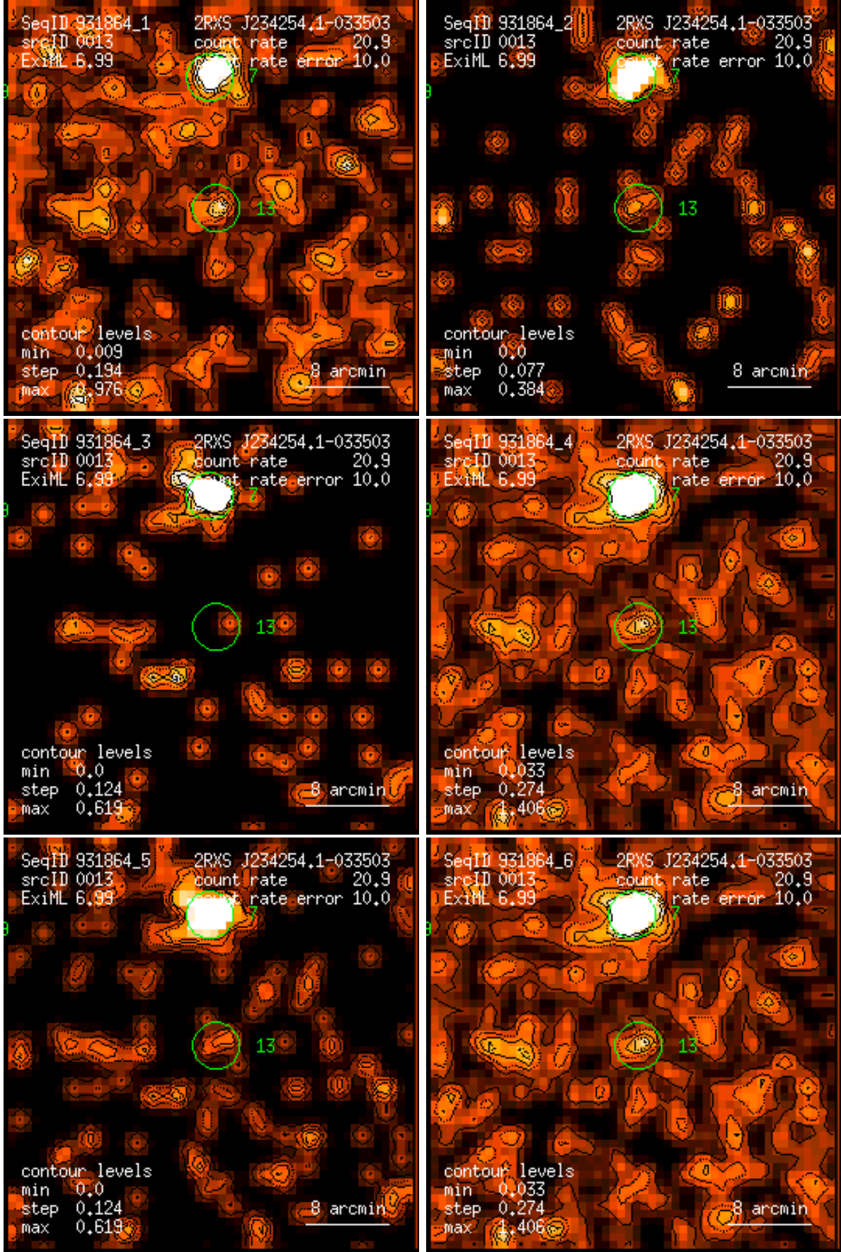
Figure 13: RASS 931864: detection 0013: band rate images, Gaussian filter: (1) PSPC channels 11 – 41, (2) 52 – 90, (3) 91 – 201, (4) 11 – 235, (5) 52 – 201, (6) 11 – 201. Broad band rates in counts/ks. Band rate contour levels in counts/ks/arcmin 2 .
