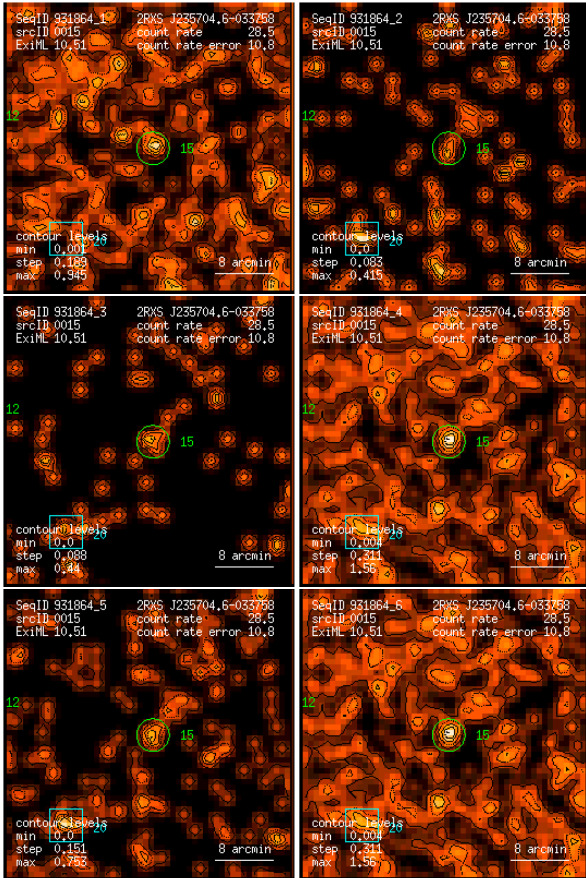
Figure 15: RASS 931864: detection 0015: band rate images, Gaussian filter: (1) PSPC channels 11 – 41, (2) 52 – 90, (3) 91 – 201, (4) 11 – 235, (5) 52 – 201, (6) 11 – 201. Broad band rates in counts/ks. Band rate contour levels in counts/ks/arcmin 2 .
