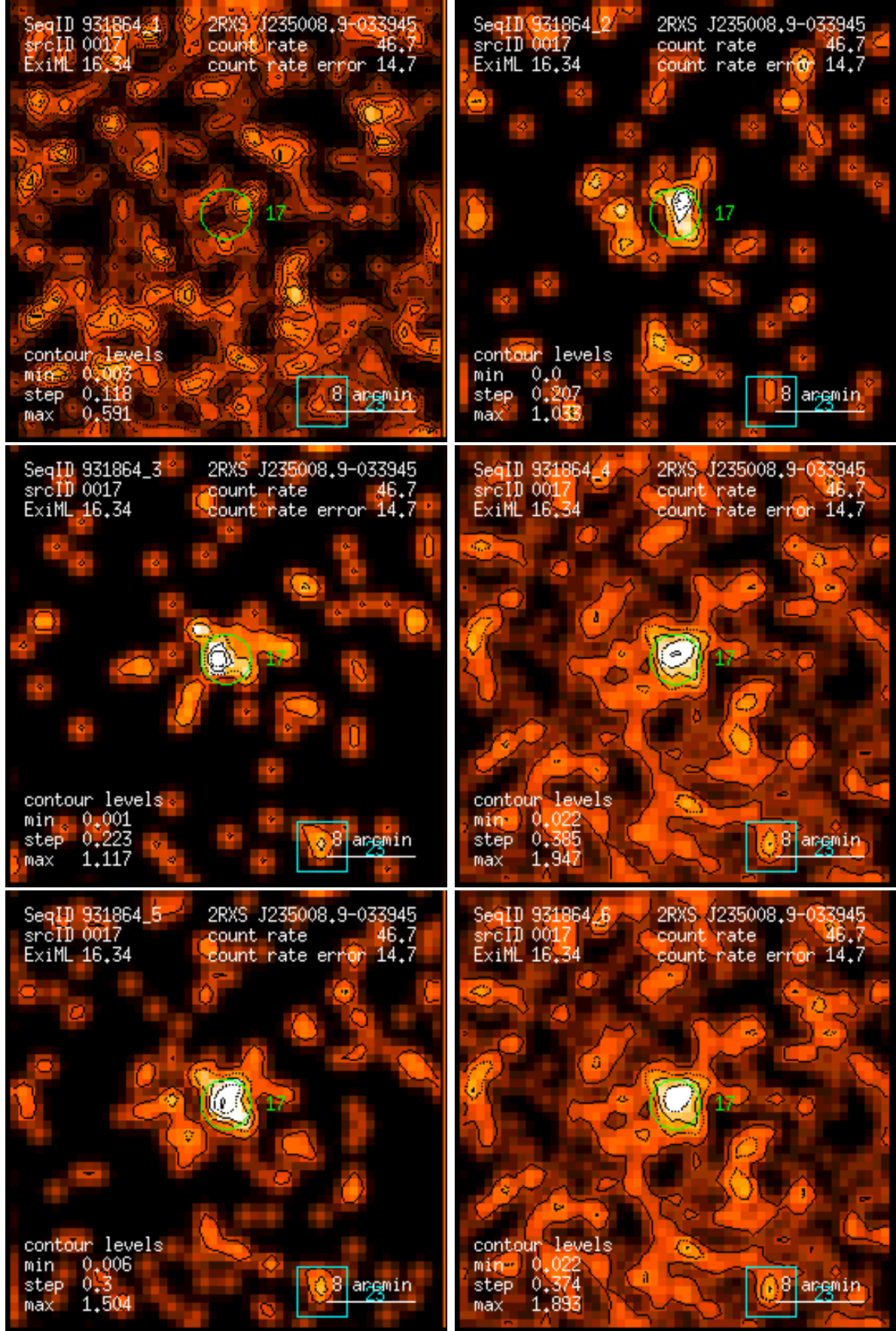
Figure 17: RASS 931864: detection 0017: band rate images, Gaussian filter: (1) PSPC channels 11 – 41, (2) 52 – 90, (3) 91 – 201, (4) 11 – 235, (5) 52 – 201, (6) 11 – 201. Broad band rates in counts/ks. Band rate contour levels in counts/ks/arcmin 2 .
