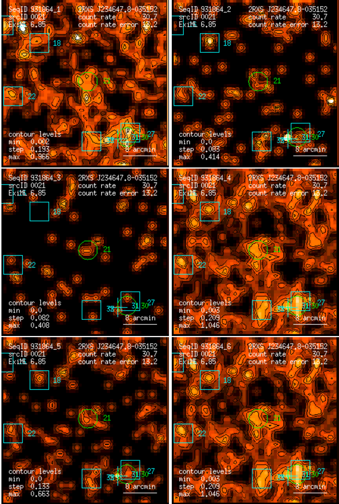
Figure 21: RASS 931864: detection 0021: band rate images, Gaussian filter: (1) PSPC channels 11 – 41, (2) 52 – 90, (3) 91 – 201, (4) 11 – 235, (5) 52 – 201, (6) 11 – 201. Broad band rates in counts/ks. Band rate contour levels in counts/ks/arcmin 2 .
