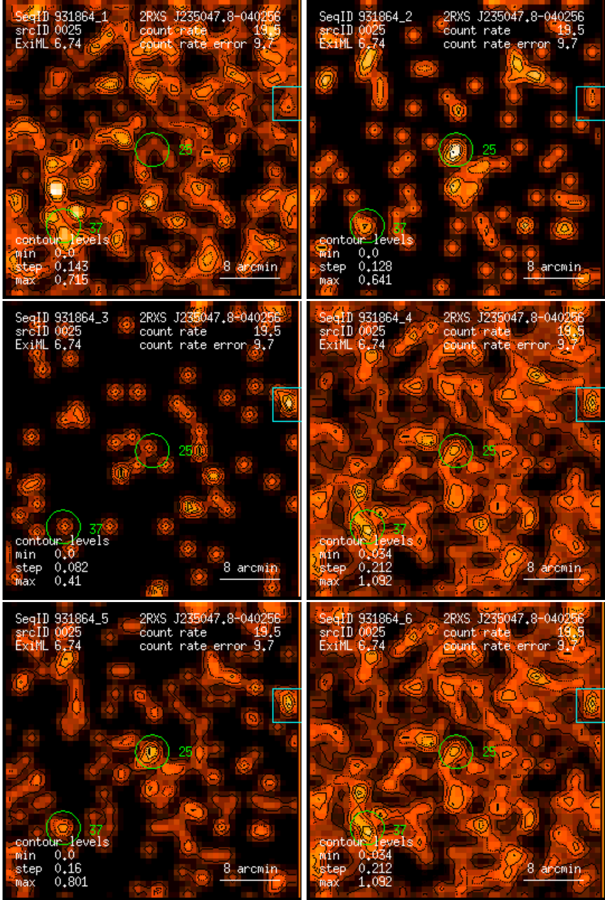
Figure 25: RASS 931864: detection 0025: band rate images, Gaussian filter: (1) PSPC channels 11 – 41, (2) 52 – 90, (3) 91 – 201, (4) 11 – 235, (5) 52 – 201, (6) 11 – 201. Broad band rates in counts/ks. Band rate contour levels in counts/ks/arcmin 2 .
