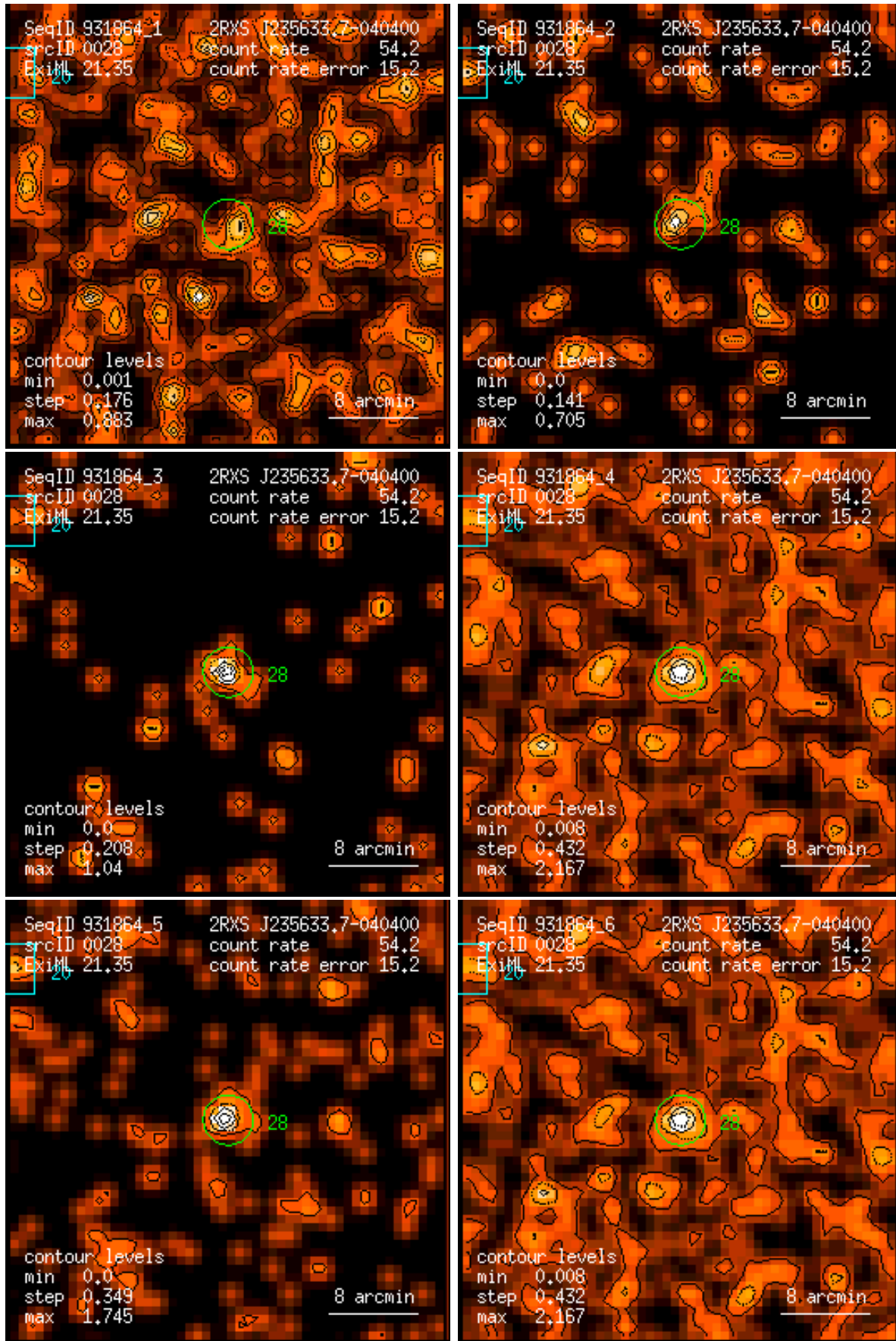
Figure 28: RASS 931864: detection 0028: band rate images, Gaussian filter: (1) PSPC channels 11 – 41, (2) 52 – 90, (3) 91 – 201, (4) 11 – 235, (5) 52 – 201, (6) 11 – 201. Broad band rates in counts/ks. Band rate contour levels in counts/ks/arcmin 2 .
