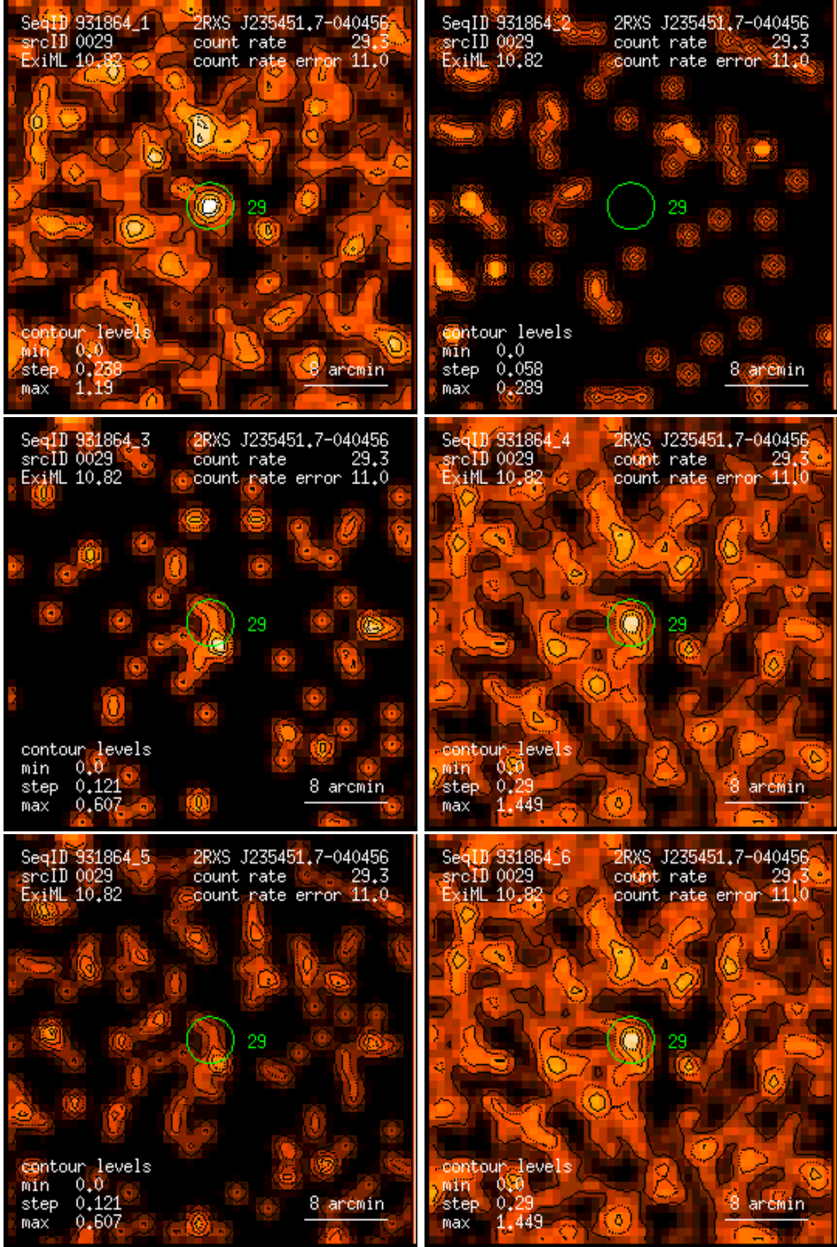
Figure 29: RASS 931864: detection 0029: band rate images, Gaussian filter: (1) PSPC channels 11 – 41, (2) 52 – 90, (3) 91 – 201, (4) 11 – 235, (5) 52 – 201, (6) 11 – 201. Broad band rates in counts/ks. Band rate contour levels in counts/ks/arcmin 2 .
