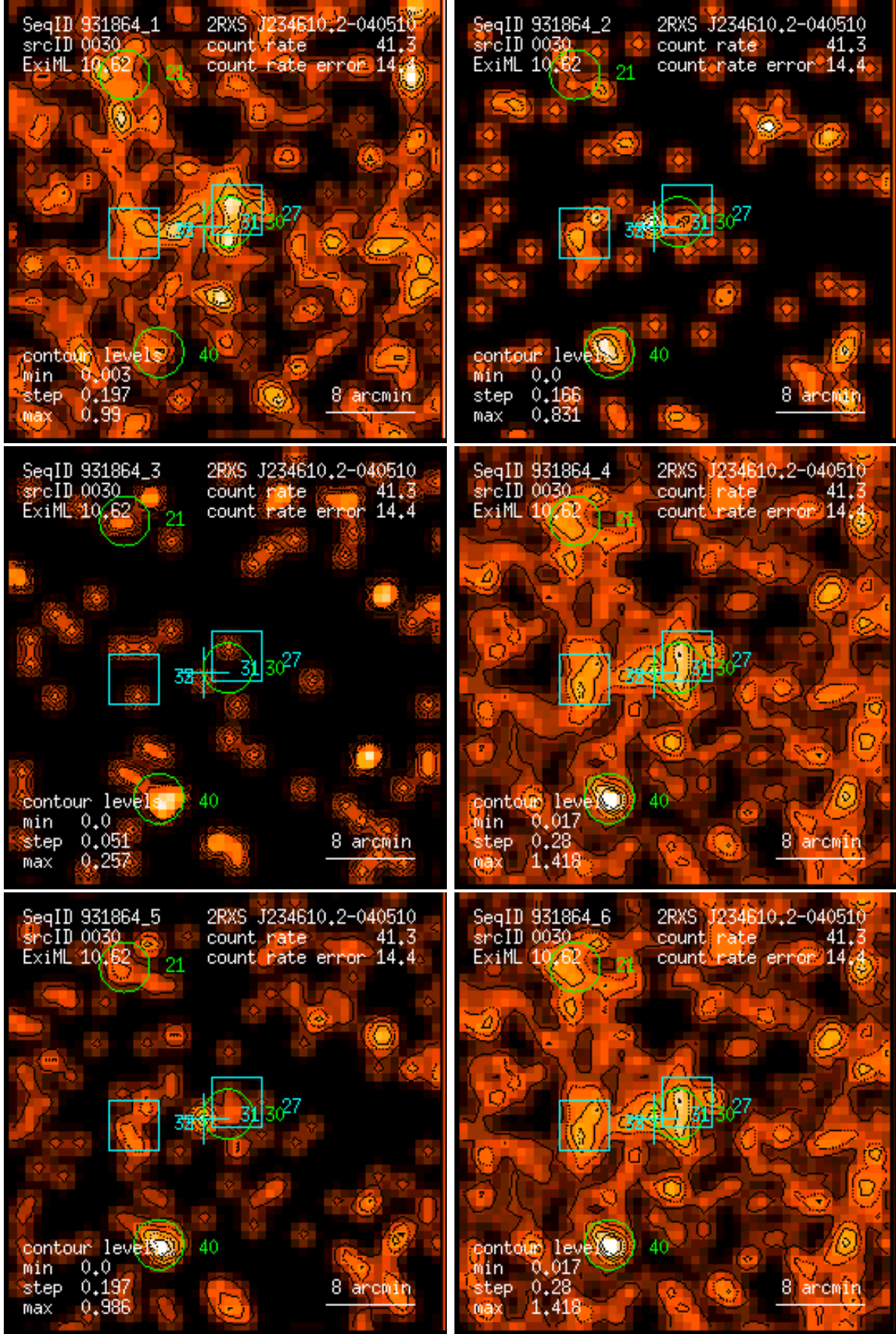
Figure 30: RASS 931864: detection 0030: band rate images, Gaussian filter: (1) PSPC channels 11 – 41, (2) 52 – 90, (3) 91 – 201, (4) 11 – 235, (5) 52 – 201, (6) 11 – 201. Broad band rates in counts/ks. Band rate contour levels in counts/ks/arcmin 2 .
