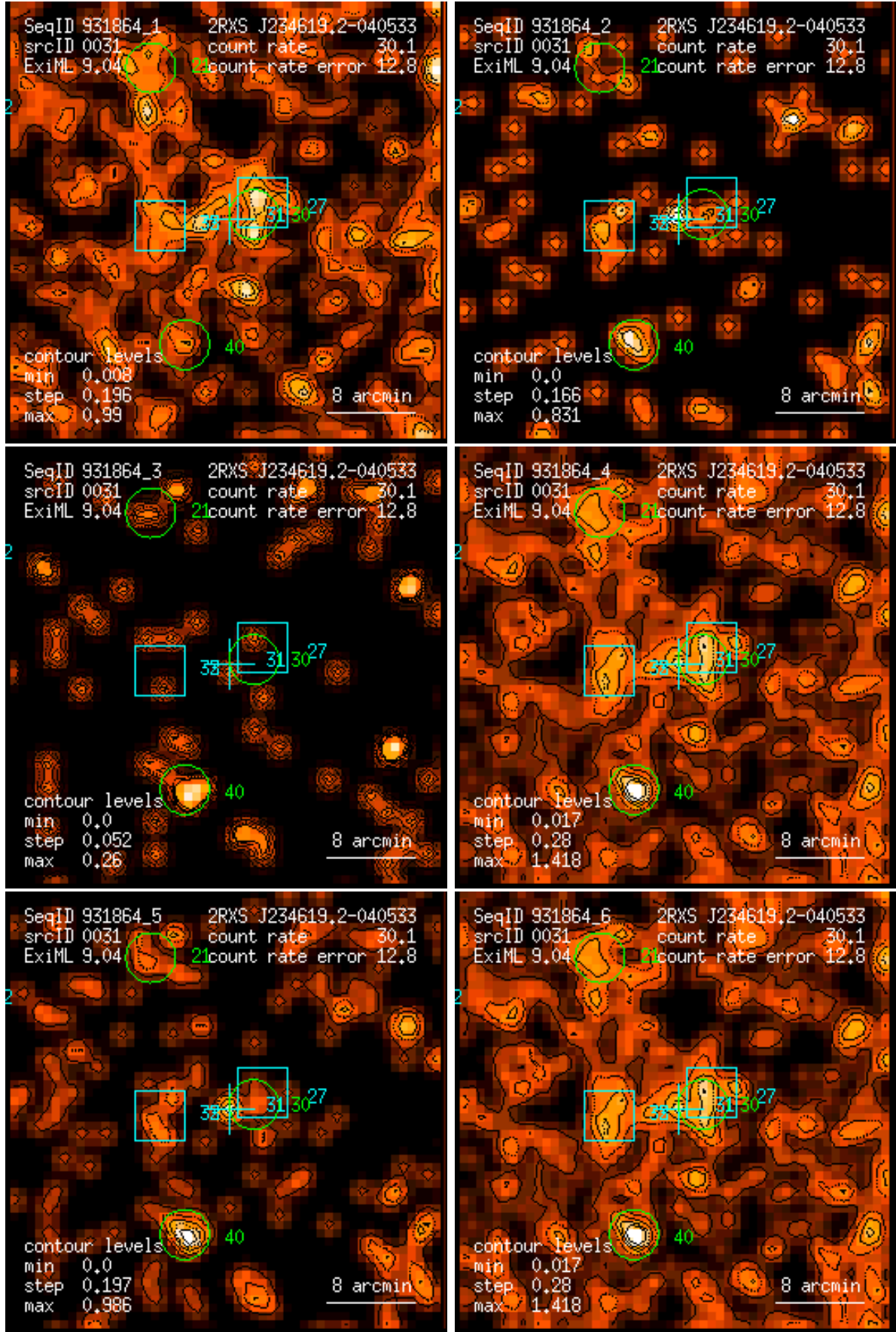
Figure 31: RASS 931864: detection 0031: band rate images, Gaussian filter: (1) PSPC channels 11 – 41, (2) 52 – 90, (3) 91 – 201, (4) 11 – 235, (5) 52 – 201, (6) 11 – 201. Broad band rates in counts/ks. Band rate contour levels in counts/ks/arcmin 2 .
