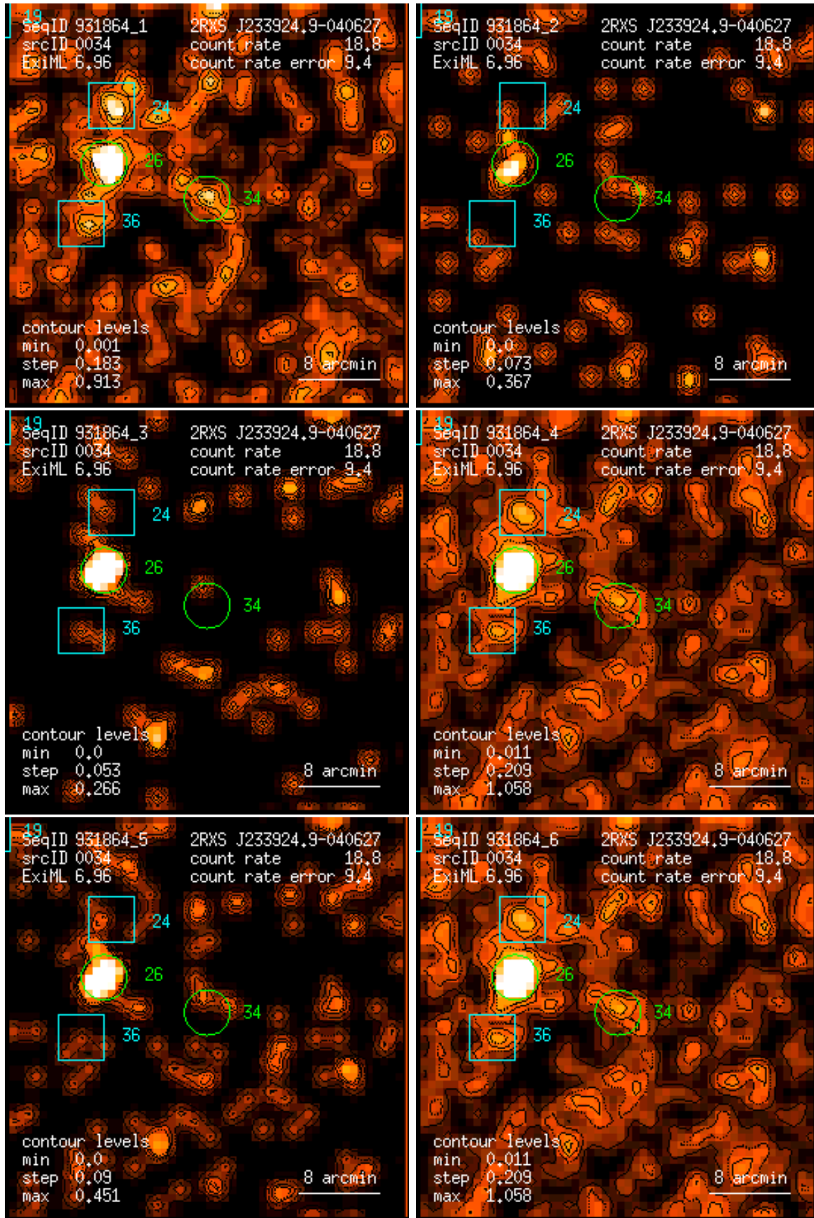
Figure 34: RASS 931864: detection 0034: band rate images, Gaussian filter: (1) PSPC channels 11 – 41, (2) 52 – 90, (3) 91 – 201, (4) 11 – 235, (5) 52 – 201, (6) 11 – 201. Broad band rates in counts/ks. Band rate contour levels in counts/ks/arcmin 2 .
