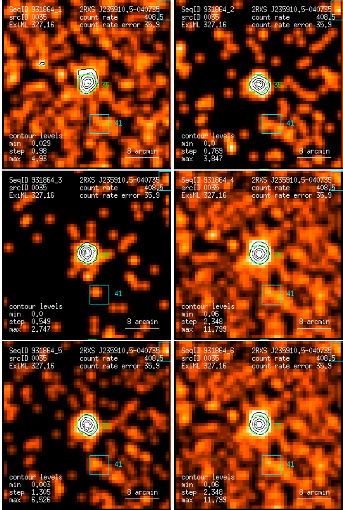
Figure 35: RASS 931864: detection 0035: band rate images, Gaussian filter: (1) PSPC channels 11 – 41, (2) 52 – 90, (3) 91 – 201, (4) 11 – 235, (5) 52 – 201, (6) 11 – 201. Broad band rates in counts/ks. Band rate contour levels in counts/ks/arcmin 2 .
