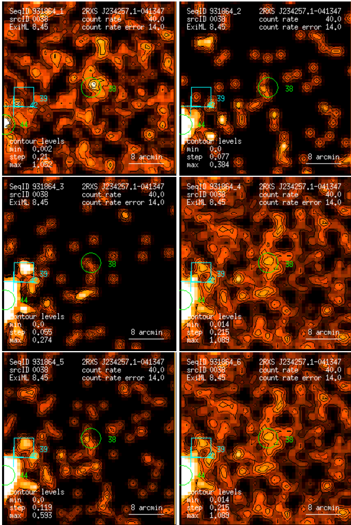
Figure 38: RASS 931864: detection 0038: band rate images, Gaussian filter: (1) PSPC channels 11 – 41, (2) 52 – 90, (3) 91 – 201, (4) 11 – 235, (5) 52 – 201, (6) 11 – 201. Broad band rates in counts/ks. Band rate contour levels in counts/ks/arcmin 2 .
