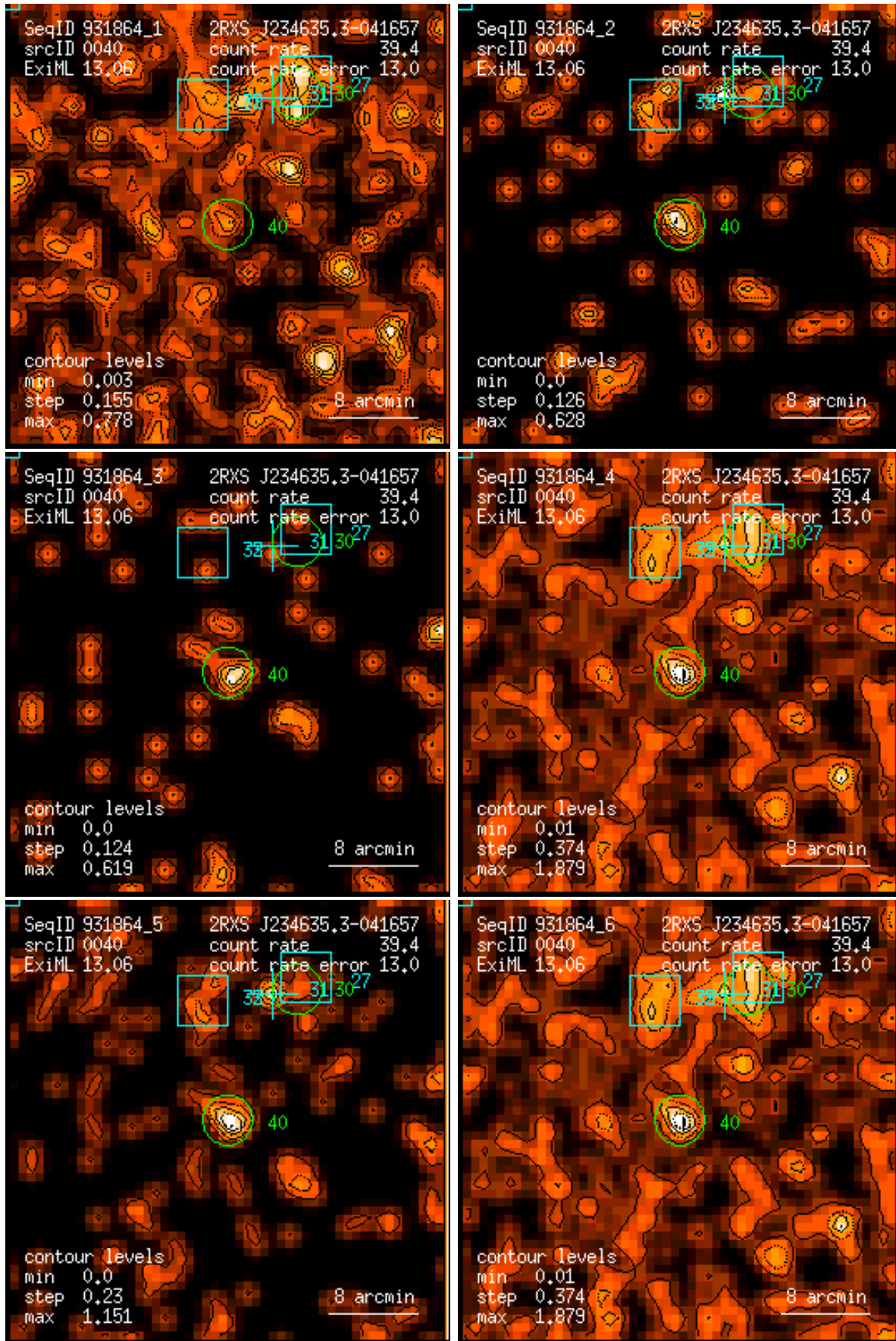
Figure 40: RASS 931864: detection 0040: band rate images, Gaussian filter: (1) PSPC channels 11 – 41, (2) 52 – 90, (3) 91 – 201, (4) 11 – 235, (5) 52 – 201, (6) 11 – 201. Broad band rates in counts/ks. Band rate contour levels in counts/ks/arcmin 2 .
