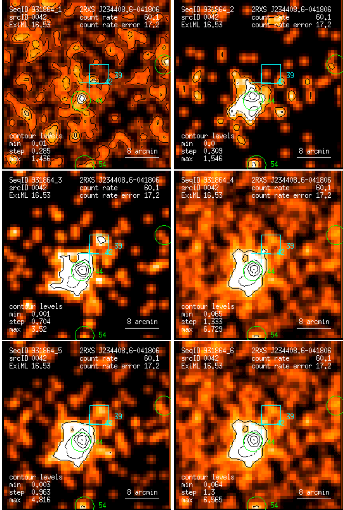
Figure 42: RASS 931864: detection 0042: band rate images, Gaussian filter: (1) PSPC channels 11 – 41, (2) 52 – 90, (3) 91 – 201, (4) 11 – 235, (5) 52 – 201, (6) 11 – 201. Broad band rates in counts/ks. Band rate contour levels in counts/ks/arcmin 2 .
