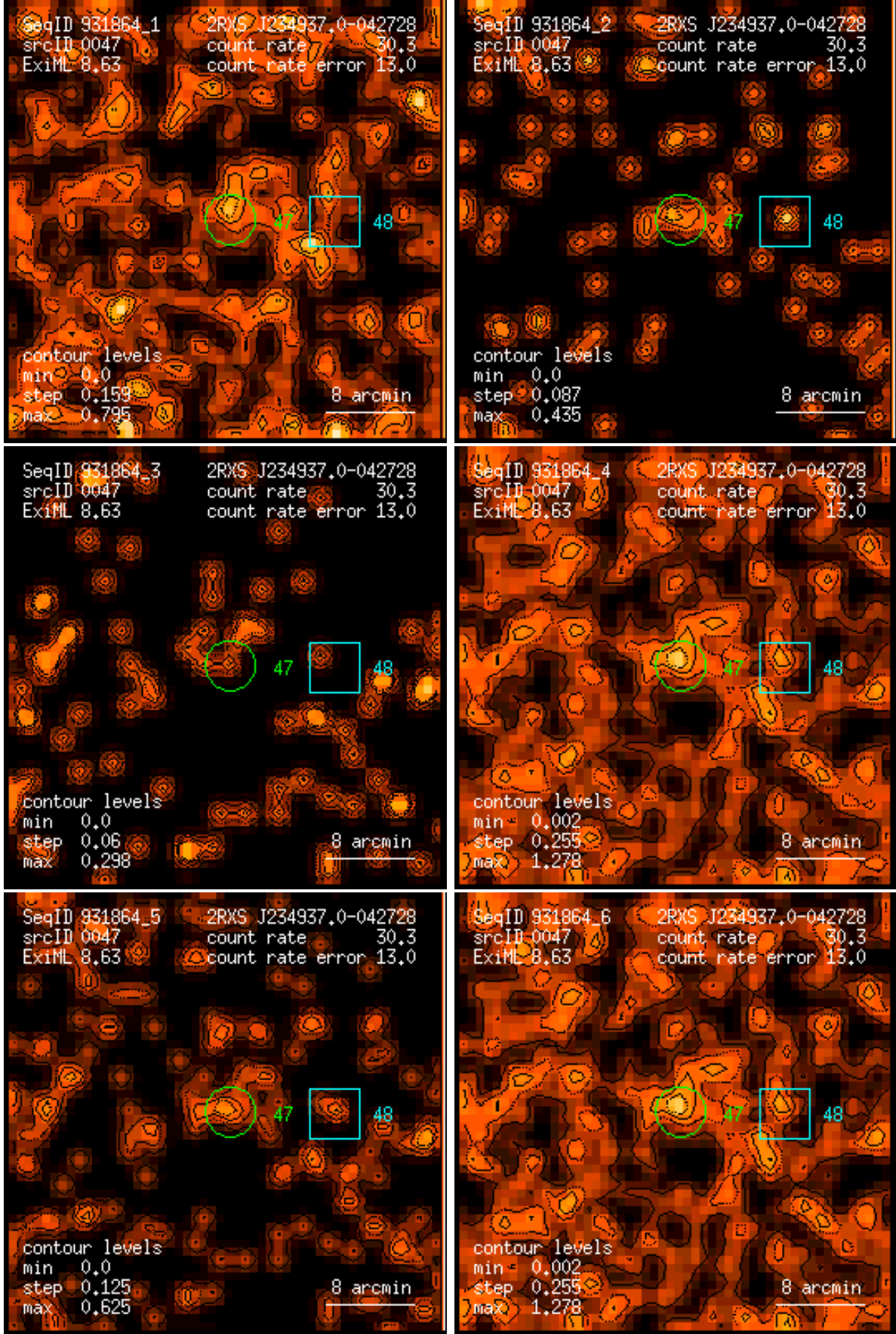
Figure 47: RASS 931864: detection 0047: band rate images, Gaussian filter: (1) PSPC channels 11 – 41, (2) 52 – 90, (3) 91 – 201, (4) 11 – 235, (5) 52 – 201, (6) 11 – 201. Broad band rates in counts/ks. Band rate contour levels in counts/ks/arcmin 2 .
