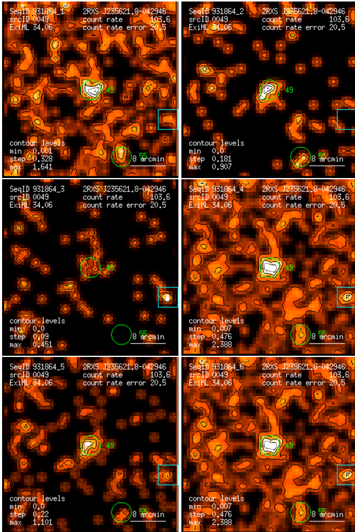
Figure 49: RASS 931864: detection 0049: band rate images, Gaussian filter: (1) PSPC channels 11 – 41, (2) 52 – 90, (3) 91 – 201, (4) 11 – 235, (5) 52 – 201, (6) 11 – 201. Broad band rates in counts/ks. Band rate contour levels in counts/ks/arcmin 2 .
