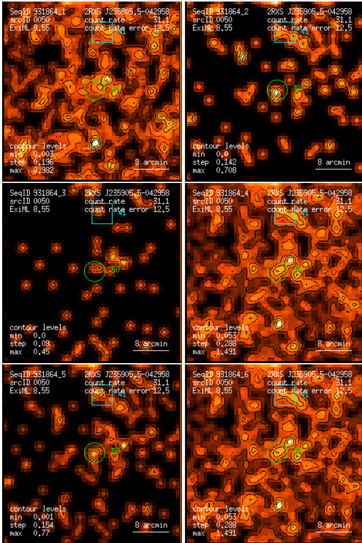
Figure 50: RASS 931864: detection 0050: band rate images, Gaussian filter: (1) PSPC channels 11 – 41, (2) 52 – 90, (3) 91 – 201, (4) 11 – 235, (5) 52 – 201, (6) 11 – 201. Broad band rates in counts/ks. Band rate contour levels in counts/ks/arcmin 2 .
