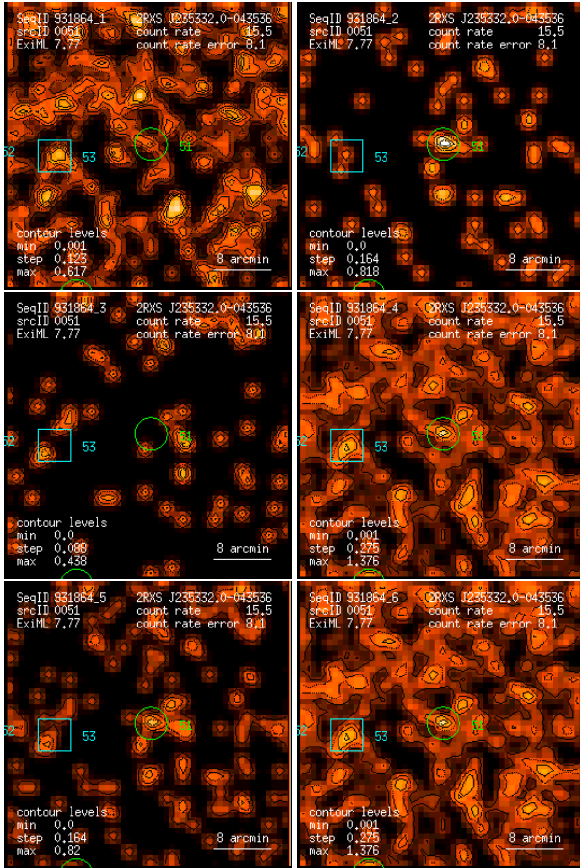
Figure 51: RASS 931864: detection 0051: band rate images, Gaussian filter: (1) PSPC channels 11 – 41, (2) 52 – 90, (3) 91 – 201, (4) 11 – 235, (5) 52 – 201, (6) 11 – 201. Broad band rates in counts/ks. Band rate contour levels in counts/ks/arcmin 2 .
