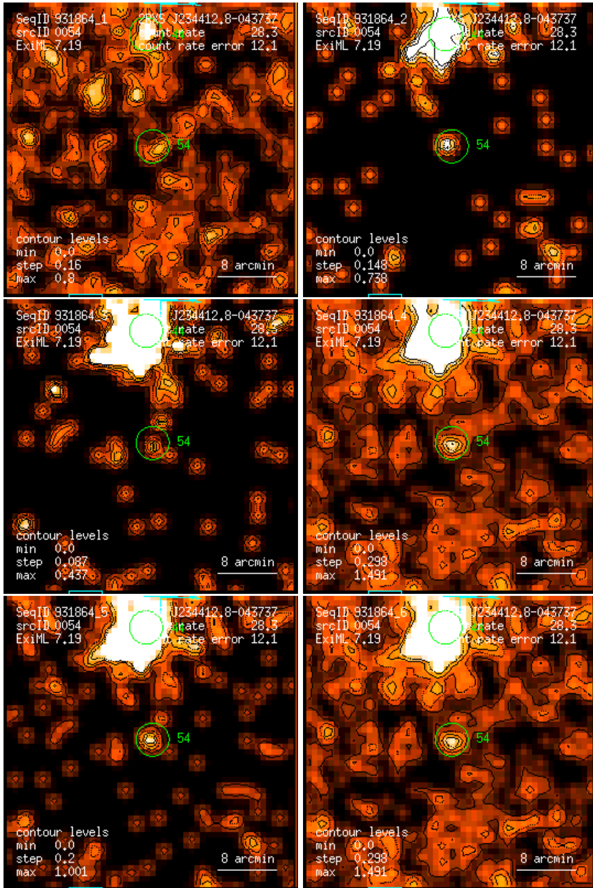
Figure 54: RASS 931864: detection 0054: band rate images, Gaussian filter: (1) PSPC channels 11 – 41, (2) 52 – 90, (3) 91 – 201, (4) 11 – 235, (5) 52 – 201, (6) 11 – 201. Broad band rates in counts/ks. Band rate contour levels in counts/ks/arcmin 2 .
