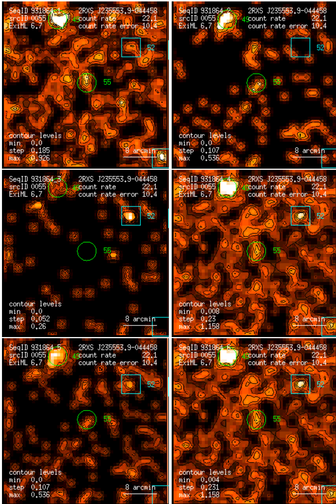
Figure 55: RASS 931864: detection 0055: band rate images, Gaussian filter: (1) PSPC channels 11 – 41, (2) 52 – 90, (3) 91 – 201, (4) 11 – 235, (5) 52 – 201, (6) 11 – 201. Broad band rates in counts/ks. Band rate contour levels in counts/ks/arcmin 2 .
