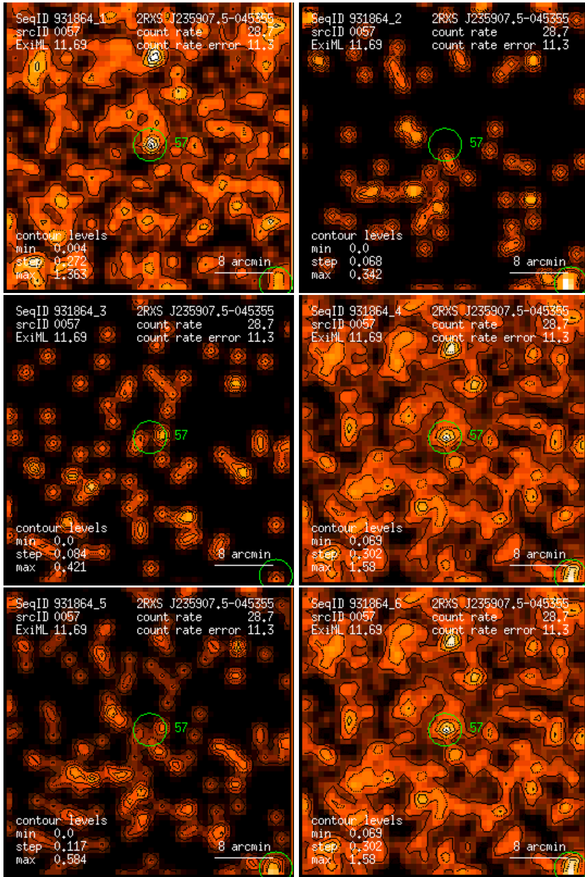
Figure 57: RASS 931864: detection 0057: band rate images, Gaussian filter: (1) PSPC channels 11 – 41, (2) 52 – 90, (3) 91 – 201, (4) 11 – 235, (5) 52 – 201, (6) 11 – 201. Broad band rates in counts/ks. Band rate contour levels in counts/ks/arcmin 2 .
