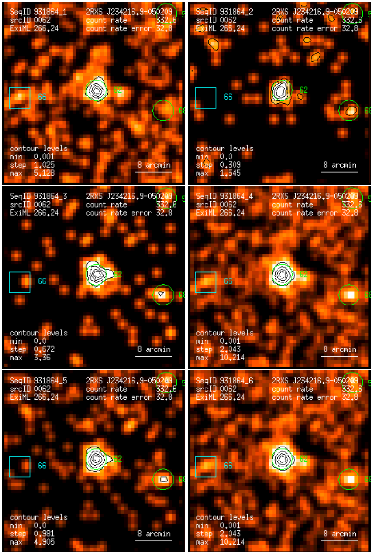
Figure 62: RASS 931864: detection 0062: band rate images, Gaussian filter: (1) PSPC channels 11 – 41, (2) 52 – 90, (3) 91 – 201, (4) 11 – 235, (5) 52 – 201, (6) 11 – 201. Broad band rates in counts/ks. Band rate contour levels in counts/ks/arcmin 2 .
